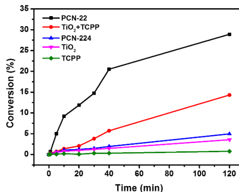
Figure 4. Time course of the benzyl alcohol oxidation reaction catalyzed by different catalyst
