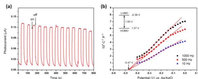
Figure 3. (a) Transient photocurrent responses of PCN-22 in 0.5 M Na 2 SO 4 aqueous solution at a bias of 0.5 V vs. Ag/AgCl under visible light irradiation; (b) Mott-Schottky plot of PCN-22 in 0.5 M Na 2 SO 4 aqueous solution.
