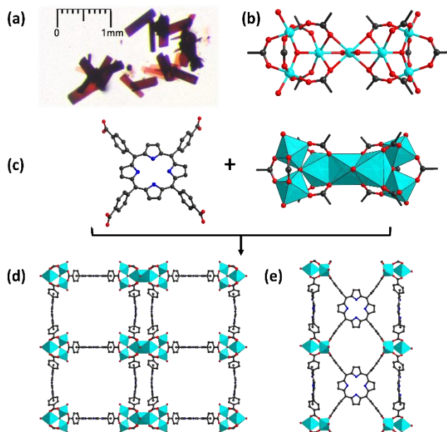
Figure 1. (a) Microscope image of PCN-22 crystals; (b) structure of the Ti 7 O 6 cluster (only O atoms of DEF molecules are shown for clarity); (c) Representation of the tetratopic TCPP linker (left) and 12-connected Ti 7 O 6 cluster (right); (d) views of the structure of PCN-22 along a -axis and (e) b -axis. Color scheme: red, O; black, C; blue, N; and cyan, Ti. H atoms are omitted for clarity.
