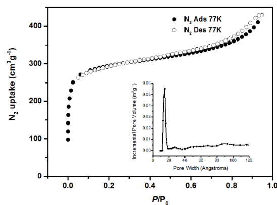
Figure 2. The N 2 adsorption isotherm of PCN-22 at 77 K, 1 atm. The inset shows DFT pore size distribution of PCN-22 using data measured with N 2 at 77 K.
