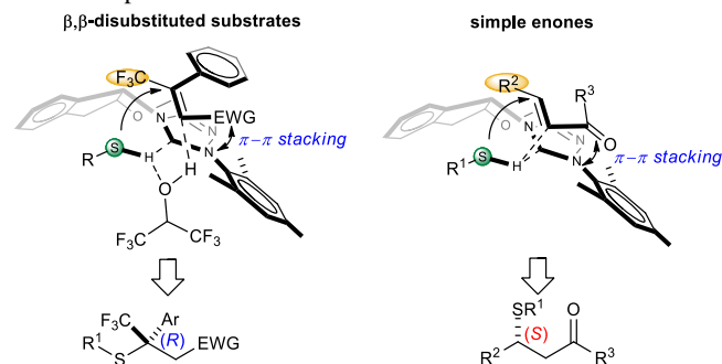
Scheme 4. Proposed model for asymmetric induction
