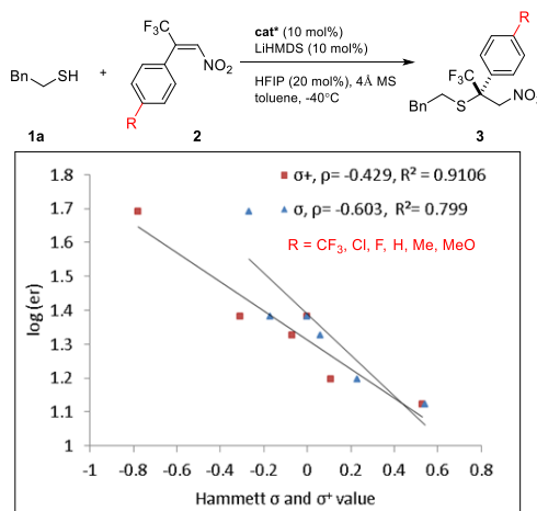
Scheme 3. LFER between substrate electronics and enantioselectivity
