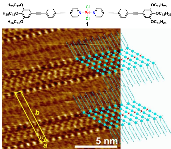
Figure 1. High-resolution STM image of the OPE-based Pd(II) complex 1 ( c = 5 \times 10^{-4} M) at the HOPG/1-phenyloctane interface and molecular packing within lamellar structures. Tunnelling condition: V_{\text{bias}} = 750 mV, I_{\text{set}} = 3.0 pA.
