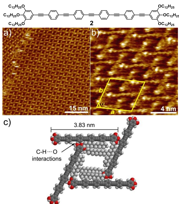
Figure 3. (a,b) STM height images of 2 at an HOPG/1-phenyloctane interface ( c = 1 \times 10^{-6} M). Z scale is 0.2 nm. Tunnelling condition: V_{\text{bias}} = 690 mV, I_{\text{set}} = 8.0 pA; (c) Proposed molecular packing of 2 within grid-like patterns in which all alkyl chains are on the HOPG surface showing C-H (aromatic)...O interactions.
