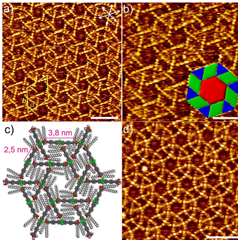
Figure 2. (a, b, d) STM height images of 1 at an HOPG/ 1 -phenyloctane interface ( c = 1 \times 10^{-6} M). Z scale is 0.2 nm. Tunnelling condition: V_{\text{bias}} = 690 mV, I_{\text{set}} = 8.0 pA. The bar scale in Figures 2a and 2d corresponds to 8 nm and in Figure 2b to 5 nm. c) Tentative space-filling model (AM1 level, Spartan) of the AT tiling showing CH \cdots Cl interactions.
