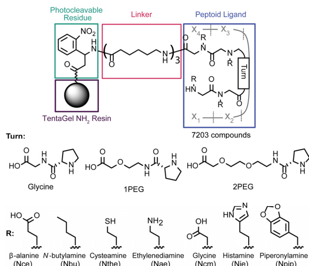
Figure 1. Peptoid library schematic. The diagram depicts the photocleavable residue, linker, and peptoid ligand structure with variable positions represented as “X n ” and “Turn”. The seven “R” residues were incorporated into each of the four peptoid positions, and the three D-Proline based turns were incorporated into the “Turn” position. The overall library consists of 7203 compounds.
