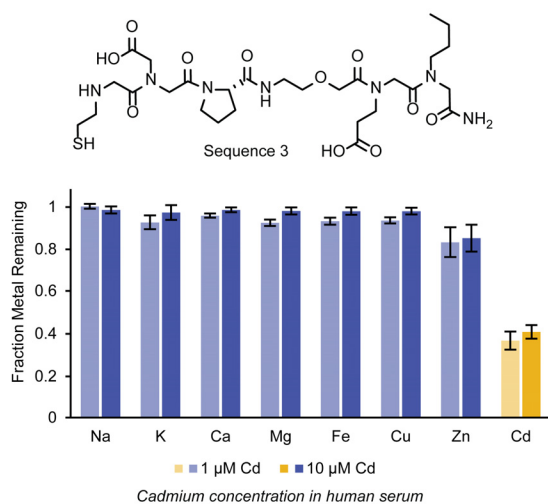
Figure 5. Evaluation of selectivity of peptoid ligands for \text{Cd}^{2+} in the presence of biological divalent cations in human serum. Two concentrations of cadmium (1 \mu\text{M} and 10 \mu\text{M} ) were exposed to Sequence 3 (100 \mu\text{M} on resin) for 24 h, and the remaining concentrations of each of the divalent cations were measured using ICP-OES. All error bars represent the standard errors of each sample set ( n = 5 ).
