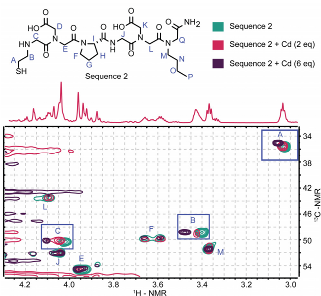
Figure 3. ^1\text{H} - ^{13}\text{C} HSQC NMR (900 MHz) spectrum of Sequence 2 (500 \mu\text{M} ) in the presence of \text{Cd}^{2+} . Resonances that shift upon the addition of \text{Cd}^{2+} are highlighted. All spectra were obtained in 10 mM phosphate buffer (pH 7) with 10% \text{D}_2\text{O} .
