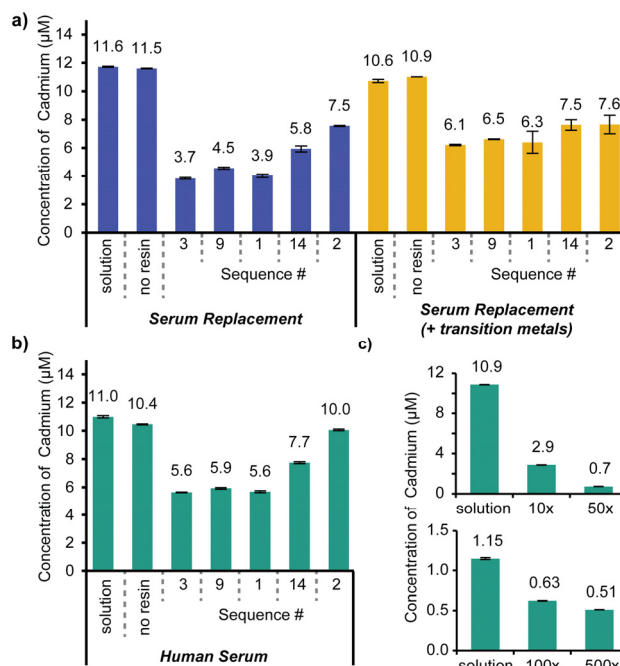
Figure 4. Evaluation of Cd 2+ binding efficacy of peptoid ligands in human serum and mimetic solutions. a) Serum replacement with and without the addition of biologically relevant transition metals (Fe 2+ , Mn 2+ , Zn 2+ , 100 μM) and b) human serum were prepared with a toxic level of Cd 2+ (10 μM) and exposed to five peptoid sequences attached to the resin (10 eq relative to Cd 2+ ). The amount of cadmium remaining after a 24 h incubation was measured with ICP-OES. The cadmium concentration in the initial solution and a sample with no resin are reported, in addition to those exposed to ligands. c) The depletion ability of Sequence 3 in human serum was additionally evaluated with more equivalents (x = eq relative to Cd 2+ ) of the ligand and at a lower concentration of Cd 2+ (1 μM). All error bars represent the standard errors of each sample set (n = 3).
