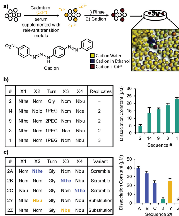
Figure 2. Overview of the screening procedure and measured Cd 2+ binding affinities of identified sequences and variants. a) An outline of the screening procedure is shown with a representative photograph of the library members after the staining procedure. The screening medium included serum replacement, added transition metal ions found free in blood (Fe 2+ , Mn 2+ , and Zn 2+ , 250 \mu M) and cadmium (25 \mu M). After incubation of the library with the screening medium, the library was rinsed and treated with cadmium dye. b) Five of the eighteen identified sequences are listed. All dissociation constants displayed were measured using titrations in HEPES buffer (10 mM, pH 7) monitored by UV-vis spectroscopy. A logistic fit was applied to the data and the inflection point was used to approximate the K d values. A 1:1 binding mode was assumed. c) Variants of the highest affinity sequence, Sequence 2, are shown. 2A–C are scrambled sequences in which the thiol containing monomer (Nthe) was switched with each residue. 2Y and 2Z are structures in which the acid containing moieties (Ncm) were replaced with Nbu to investigate the significance of each residue. The binding was characterized using the same method as (b); however, for Z, the affinity was too low to measure. All error bars represent the standard error of the logistic fit.
