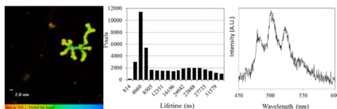
Fig. 3. Phosphorescence lifetime image map focussing on a representative extracellular feature in samples taken immediately after the introduction of Geobacter sulfurreducens to uranyl acetate solution (left), a histogram showing the distribution of lifetime measurements (centre), and a representative, uranyl spectrum from one such extracellular feature (right) ( \lambda_{ex} = 405 nm, room temperature).
