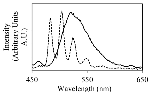
Fig. 1. Emission spectra of the uranyl cation in a carbonate buffer solution (30 mmol) in the presence of Geobacter sulfurreducens at room temperature (solid line) and 77 K (dotted line), ( \lambda_{ex} = 420 nm).
