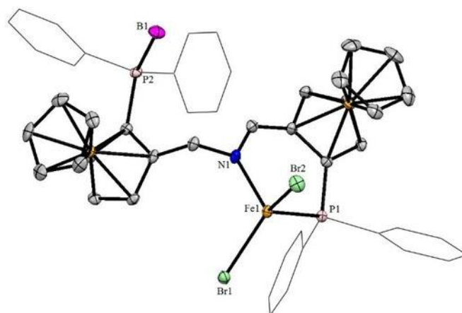
Figure 7. Structural view of (S_{Fc},S_{Fc}) - 14 showing 50% thermal ellipsoids (selected H atoms and solvent molecules are omitted for clarity). Selected bond lengths ( \text{\AA} ) and bond angles ( ^\circ ): Fe1–Br1 2.3911(7), Fe1–Br2 2.3887(6), Fe1–P1 2.400(1), Fe1–N1 2.088(3), P2–B1 1.927(5), Br1–Fe1–Br2 117.74(3), P1–Fe1–Br1 110.70(3), P1–Fe1–Br2 112.80(3), Br1–Fe1–N1 115.53(9), Br2–Fe1–N1 102.68(9).
