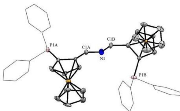
Figure 1. Structural view of (S_{Fc},S_{Fc}) - 1a showing 50 % thermal ellipsoids (H atoms and solvent molecules are omitted for clarity). Selected bond lengths (Å) and bond angles (°): C1A–N1 1.29(1), C1B–N1 1.40(1), C1A–N1–C1B 117.5(8).
