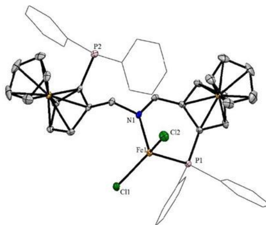
Figures 3. Structural view of (S_{Fc},S_{Fc}) - 13c showing 50% thermal ellipsoids (H atoms and solvent molecules are omitted for clarity). Selected bond lengths (Å) and bond angles (°): Fe1–Cl1 2.2438(8), Fe1–Cl2 2.2472(8), Fe1–P1 2.4031(8), Fe1–N1 2.095(2), Cl1–Fe1–Cl2 119.83(3), P1–Fe1–Cl1 110.96(3), P1–Fe1–Cl2 112.63(3), Cl1–Fe1–N1 113.32(7), Cl2–Fe1–N1 106.64(7).
