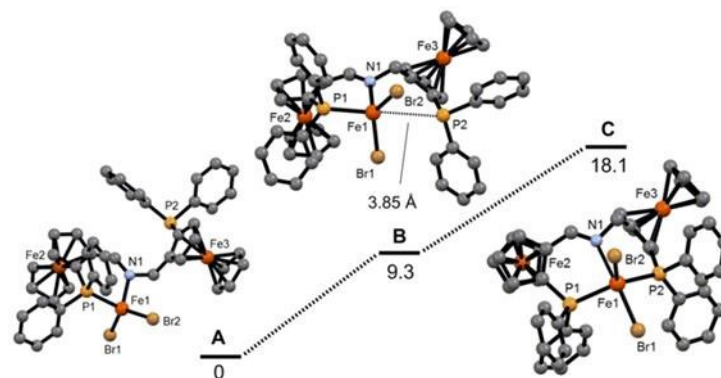
Figure 5. Free energies (B3LYP) of optimized iron PNP complexes featuring \kappa^2P,N and \kappa^3P,N,P -bound PNP ligands. The free energy values (kcal/mol) are referred to the experimentally obtained tetrahedral [\text{Fe}(\kappa^2P,N\text{-PNP})\text{Br}_2] ( S_{\text{Fc}},S_{\text{Fc}} )- 13a ( A ).
