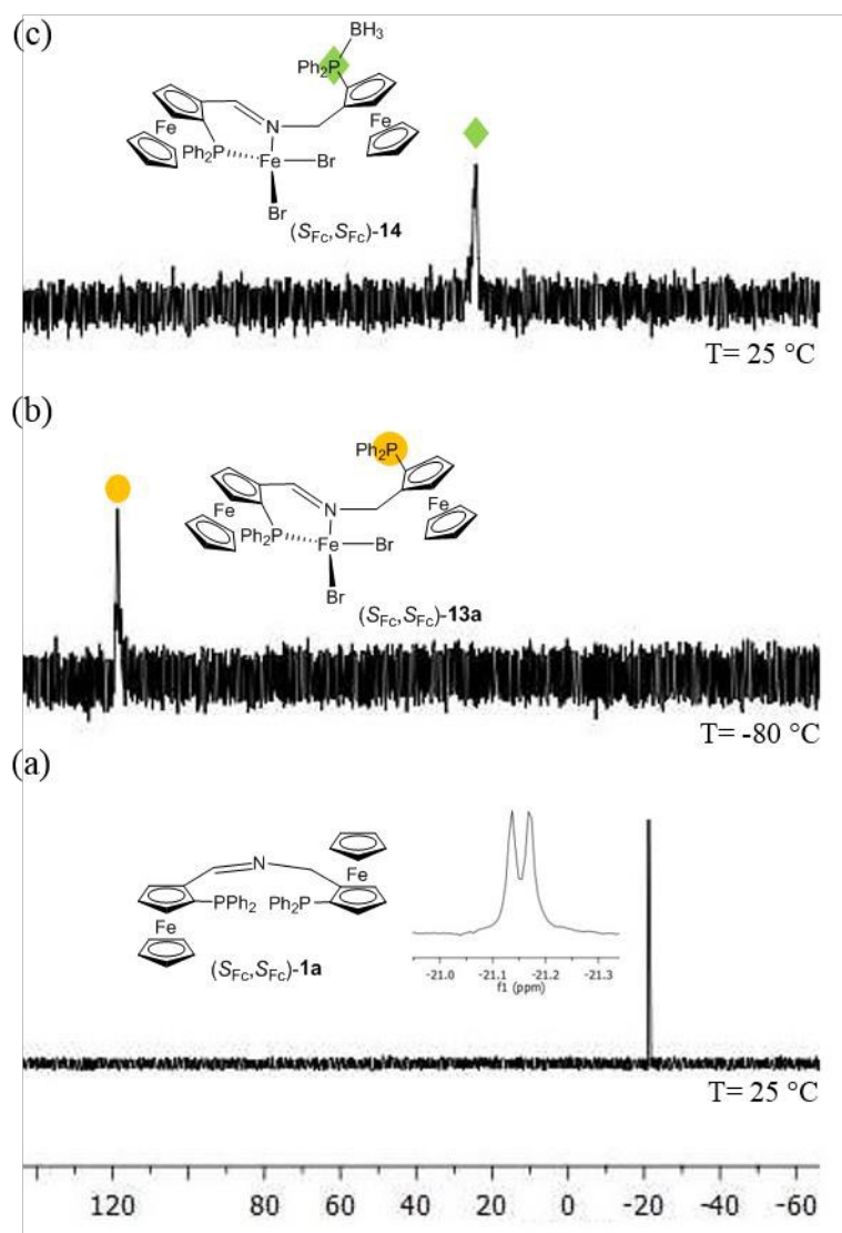
Figure 6. ^{31}\text{P}\{^1\text{H}\} NMR spectra of (a) (S_{\text{Fc}},S_{\text{Fc}})\text{-1a} , (b) \text{Fe}(\kappa^2P,N\text{-PNP})\text{Br}_2 (S_{\text{Fc}},S_{\text{Fc}})\text{-13a} at -80\text{ }^\circ\text{C} , and (c) \text{Fe}(\kappa^2P,N\text{-PNP})\text{Br}_2 (S_{\text{Fc}},S_{\text{Fc}})\text{-14} in \text{CD}_2\text{Cl}_2 (spectra of (S_{\text{Fc}},S_{\text{Fc}})\text{-13a} and (S_{\text{Fc}},S_{\text{Fc}})\text{-14} are referenced internally to \text{PPh}_3 set to -5.6\text{ ppm} ).
