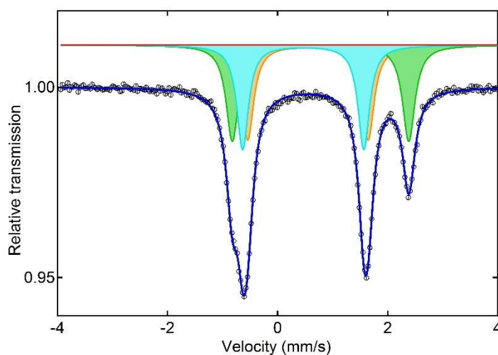
Figure 4. ^{57}\text{Fe} Mössbauer spectrum of [Fe( \kappa^2P,N -PNP)Br 2 ] ( S_{\text{Fe}}, S_{\text{Fe}} )- 13a collected at 78 K.
