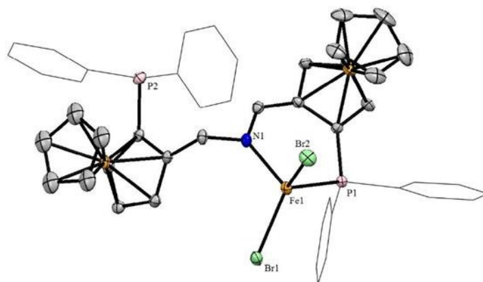
Figures 2. Structural view of ( S_{Fc},S_{Fc} )- 13a showing 50% thermal ellipsoids (H atoms and solvent molecules are omitted for clarity). Selected bond lengths (Å) and bond angles (°): Fe1–Br1 2.3818(5), Fe1–Br2 2.3916(5), Fe1–P1 2.3999(9), Fe1–N1 2.090(3), P1–Fe1–Br1 110.42(3), P1–Fe1–N1 95.16(8), Br1–Fe1–N1 115.47(8), Br2–Fe1–P1 112.84(3), Br2–Fe1–N1 102.08(8).
