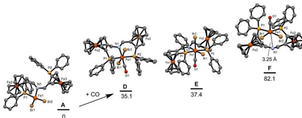
Figure 8. Free energy profile (B3LYP) for the addition of CO to form the illusive complexes trans -P, trans -Br-[Fe(PNP)(CO)Br 2 ] ( S_{Fc},S_{Fc} )- 15a ( D ), cis -Br, trans -P-[Fe(PNP)(CO)Br 2 ] ( S_{Fc},S_{Fc} )- 15a ( E ) and cis -Br, cis -P-[Fe(PNP)(CO)Br 2 ] ( S_{Fc},S_{Fc} )- 15a ( F ). The energy values (kcal/mol) are referred to [Fe( \kappa^2 P,N-PNP)Br 2 ] ( S_{Fc},S_{Fc} )- 13a ( A ).
