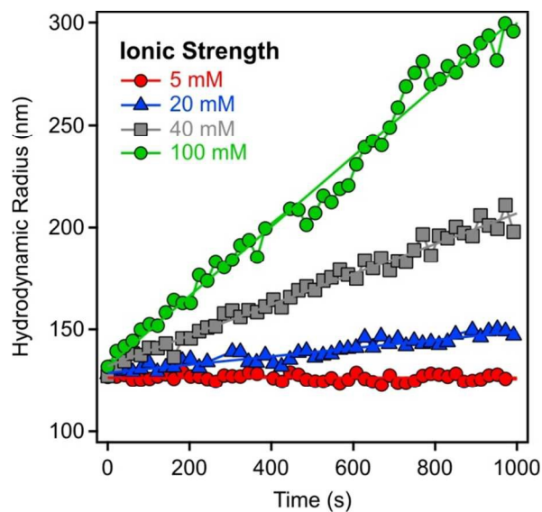
Fig. 1 Hydrodynamic radii of LDH1 particles versus time measured in time-resolved DLS experiments at 9.3 mg/L particle concentration and different ionic strengths adjusted with NaCl.
