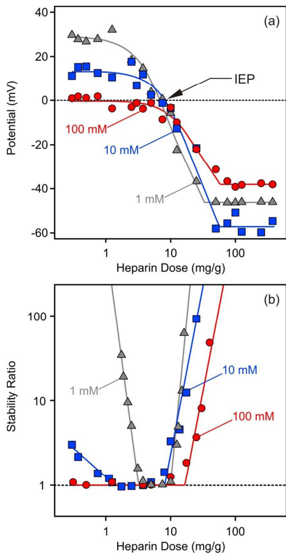
Fig. 5 Electrokinetic potential (a) and stability ratio (b) values for LDH2 in the presence of heparin at different ionic strengths. The mg/g unit refer to mg heparin per gram of LDH. The lines are just to guide the eyes.
