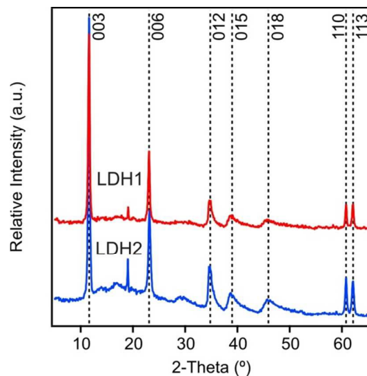
Fig. 2 Powder XRD pattern of the LDH particles, composed of magnesium(II) and aluminium(III) cations and carbonate interlayer anions, synthesized by coprecipitation. The peak at 19^\circ could be due to the 001 peak of \text{Mg}(\text{OH})_2 that was formed from soluble magnesium(II) and hydroxide ions after drying.
