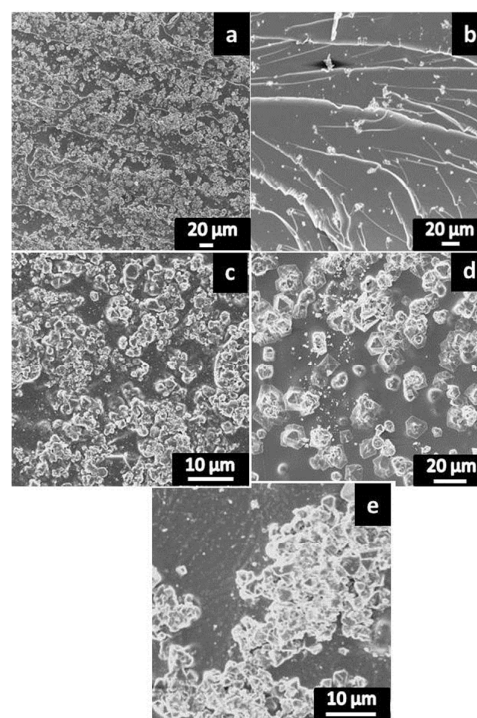
Figure 2. SEM micrographs of the surface (a, c, d, e) and cross-section (b) of polymer-MOF composites based on MMA/PEGDMA (a, b, d) and VA/PEGDMA (c, e) with different M:XL mol. ratio; a, b, d - 1:1 and c, e, 3:1.
