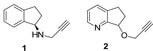
Figure 1. ( R )-Rasagiline ( 1 ) and a rasagiline analogue, 7-(1-pyrindanyl) propargyl ether ( 2 ).
