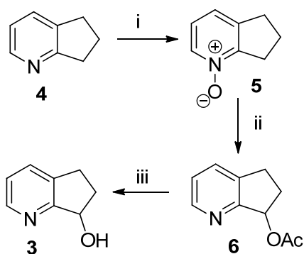
Scheme 1. Optimized synthesis of alcohol 3 . 6 Reagents and conditions: (i) m -CPBA, \text{CH}_2\text{Cl}_2 , r. t., 2 h, 99%; (ii) \text{Ac}_2\text{O} , 100^\circ\text{C} , 2h, 72%; (iii) \text{KOH} , \text{EtOH} , r. t., 1 h, 90%.
