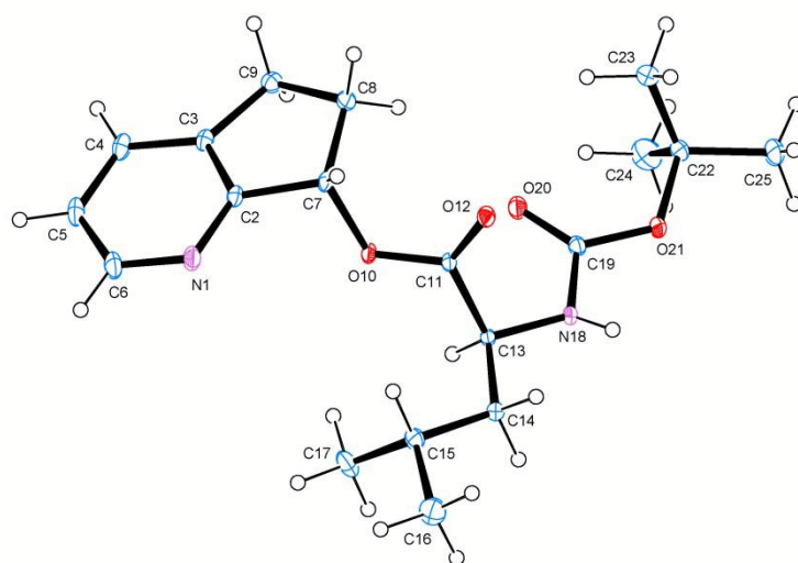
Figure 2. X-ray crystallographic structure of compound 9 .
