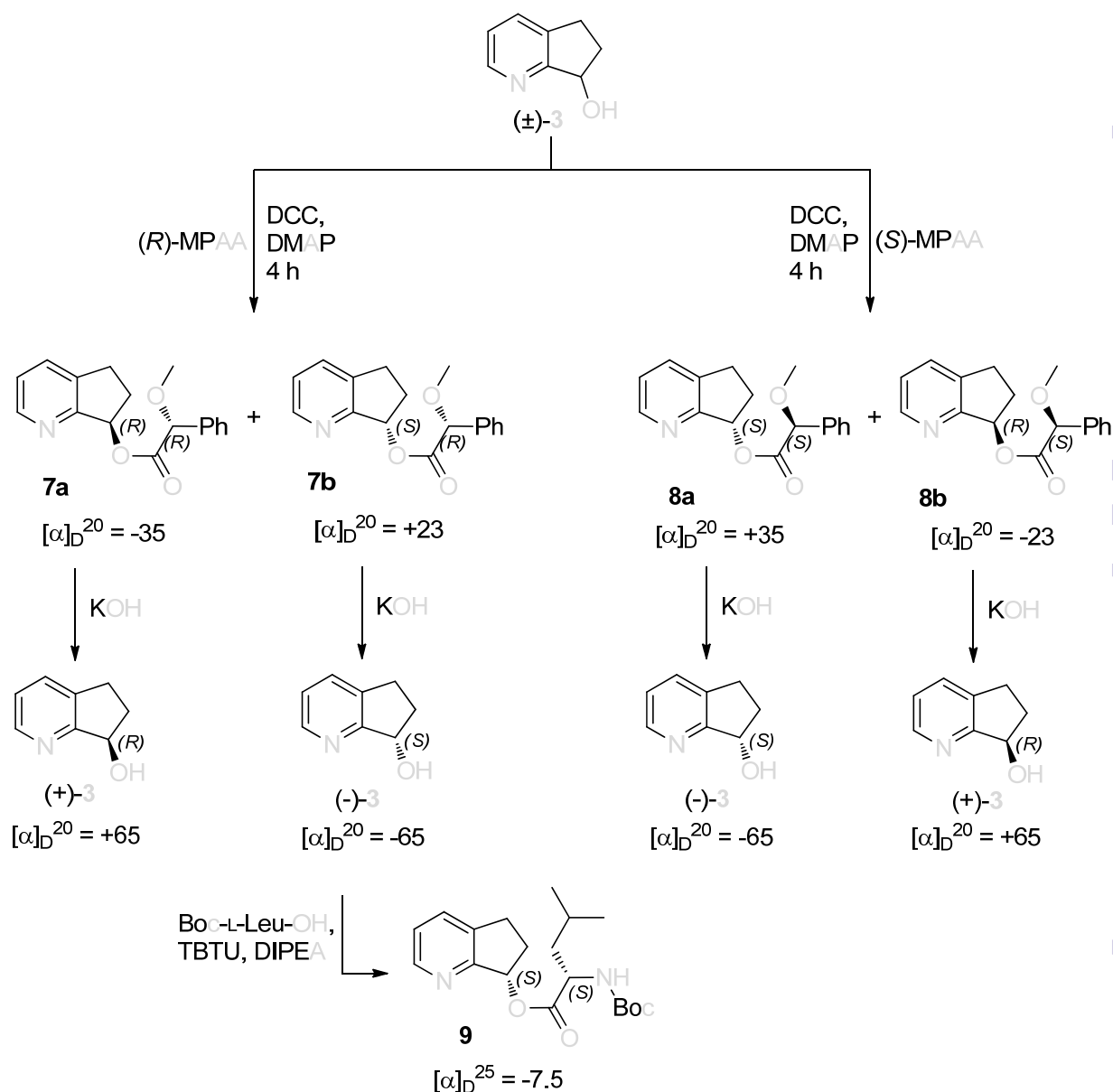
Scheme 2. Procedure for chemical resolution of (\pm)\text{-3} using (R)\text{-MPAA} and (S)\text{-MPAA} as resolution agents.
