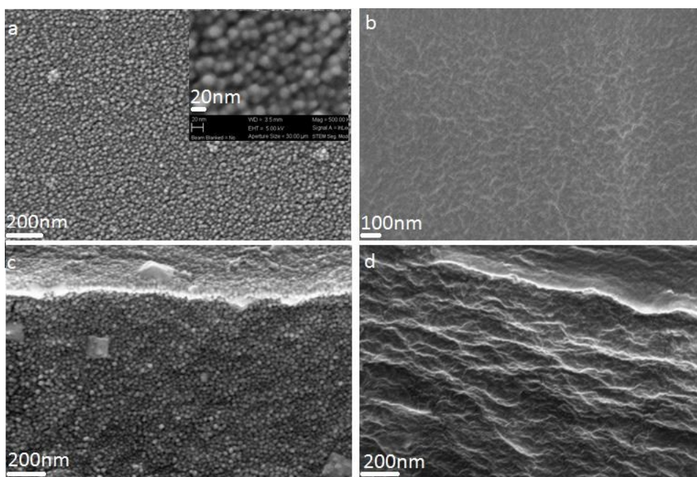
Figure 11: Top and cross-section FESEM views of the UV patterned sample: a) and c) UV irradiated part, while b) and d) non-irradiated part. The inset to the part a) shows the top view at higher magnification to present the close distribution and sizes of the Ag NPs.
