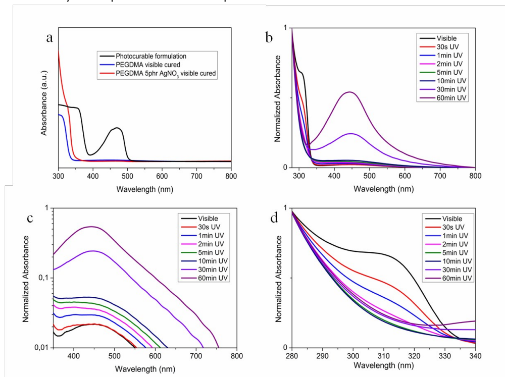
Figure 3 UV-Visible spectra: a) comparison of uncured PEGDMA formulation, PEGDMA and PEGDMA + 5phr \text{AgNO}_3 after visible-light induced curing; b) growth kinetics of Ag NPs under UV-light at different irradiation times; c) Log-scale graph of the visible part of graph b; d) UV-component of graph b
