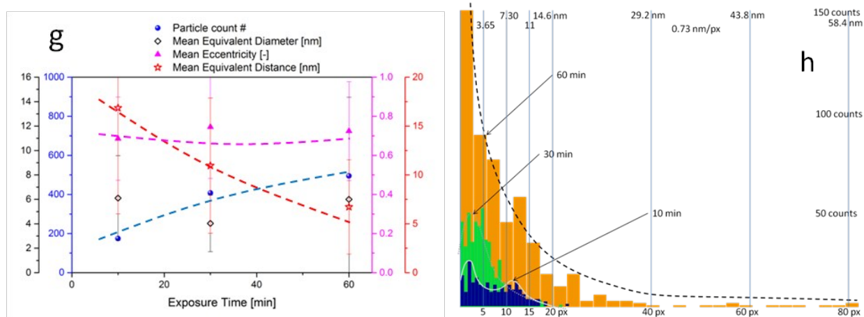
Figure 5 Top view FESEM images PEGDMA containing 5 phr \text{AgNO}_3 after: a, b) 10, c, d) 30 and e, f) 60 min of UV irradiation. The images in the right column (b, d and f) are higher magnification of those in the left column (a, c and e). g) numerical analysis of the same images; h) size distribution histograms. Lines are providing the trend and do not represent any fit.
