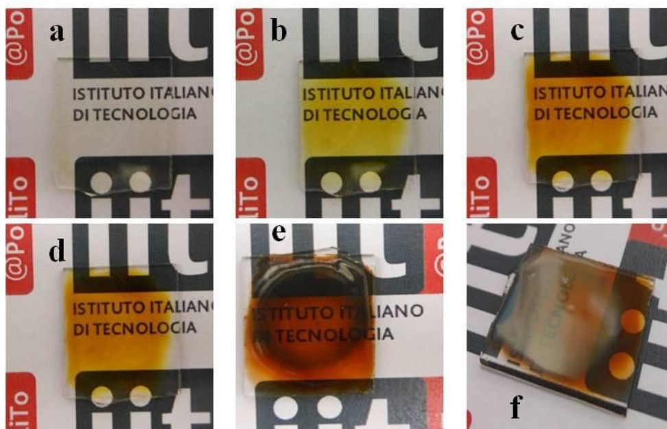
Figure 4 Images of PEGDMA containing 5 phr \text{AgNO}_3 a) after visible-light induced polymerization; b) –e) after different UV irradiation time (1 min, 10 min, 30 min and 60 min respectively); f) reflected light view of PEGDMA + 5 phr \text{AgNO}_3 after 60 minutes UV irradiation.
