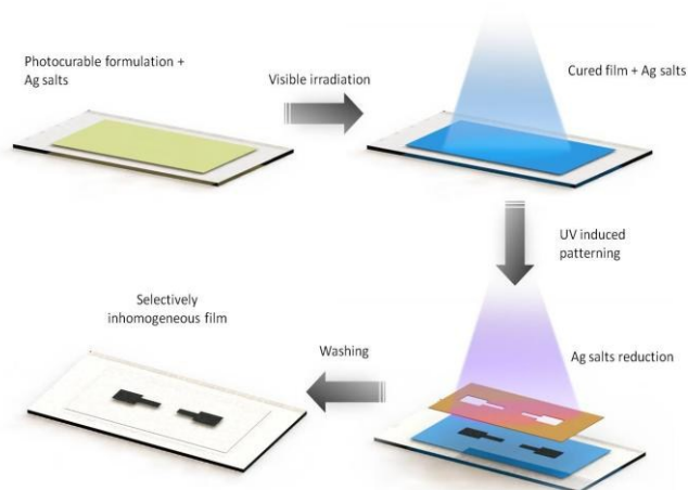
Figure 1 Process layout for the realization of selectively patterned films by dual step irradiation process: in the first step a photocurable formulation containing silver nitrate is cross-linked by means of visible light irradiation, then patterned structures of Ag NPs are generated in the polymeric matrix by UV reduction exploiting photolithography; finally unreduced ions are extracted by means of ethanol washing.
