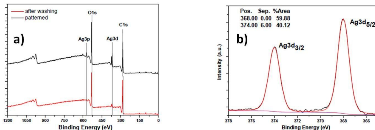
Figure 8 a) XPS survey spectra of patterned sample (black line) and un-patterned region after washing procedure (red line). b) Ag3d doublet HR spectrum of patterned sample with deconvolution parameters obtained after Shirley background subtraction and mixed Gauss-Lorentz curve fitting.
