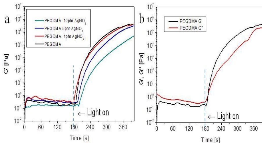
Figure 2 (a) Time dependence of G' at 25 °C and 1 rad/s for the visible light polymerization process of PEGDMA in the presence of different quantities of silver nitrate. Dotted line indicates the turning on of the lamp after 3 minutes from the beginning of the measurement. (b) Time dependence of G' and G'' for sample PEGDMA reported as example, the gel point is obtained from intersection point of G' and G'' .
