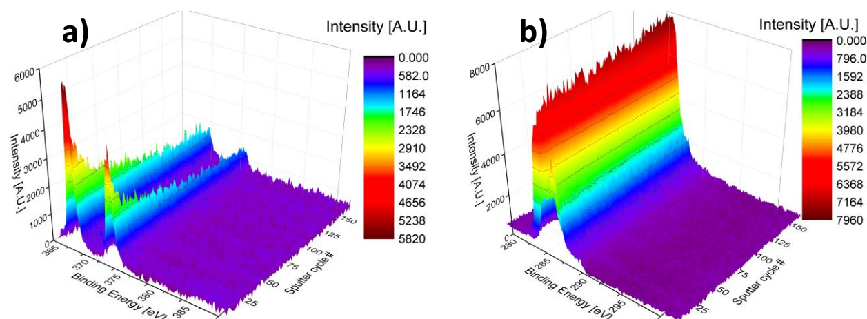
Figure 9 a) XPS Ag3d doublet and b) C1s HR spectra of patterned sample during depth profile analysis (160 cycles)
