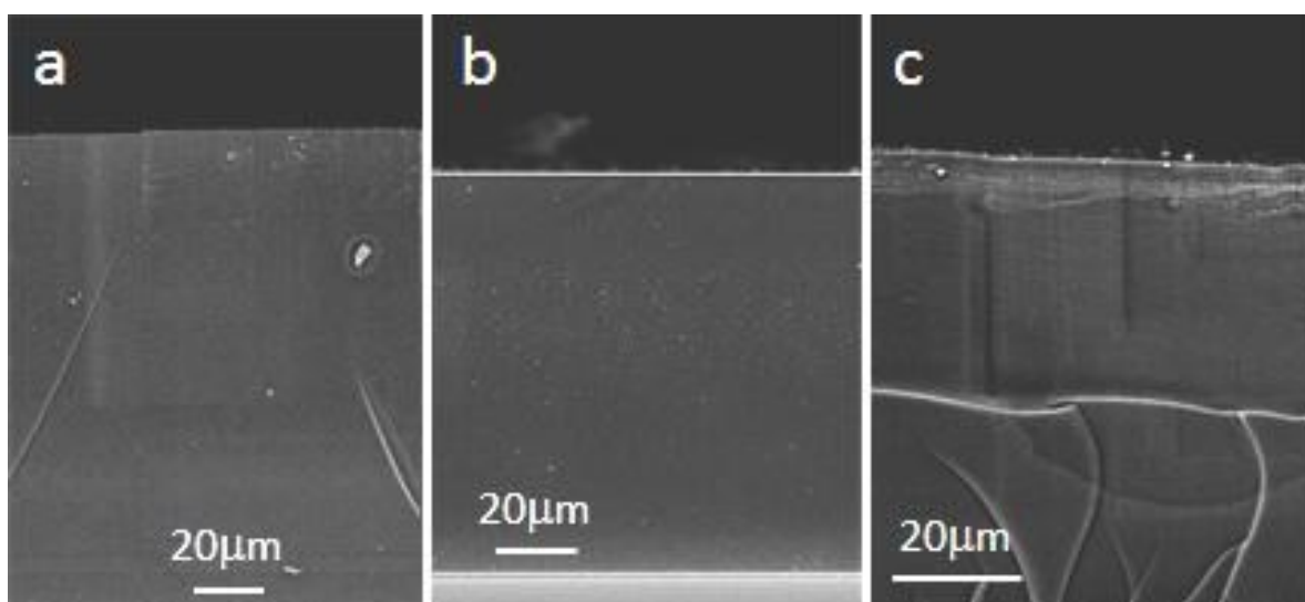
Figure 6. Cross-section FESEM images of PEGDMA containing 5 phr \text{AgNO}_3 after: a) 10, b) 30 and c) 60 min of UV irradiation.
