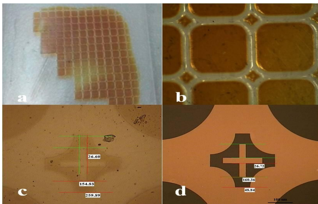
Figure 10. Picture of patterned PEGDMA + 5 phr \text{AgNO}_3 after washing step a) full film b) detail c) optical microscopy (100x) of the patterned structure d) optical picture of the mask used for the patterning
