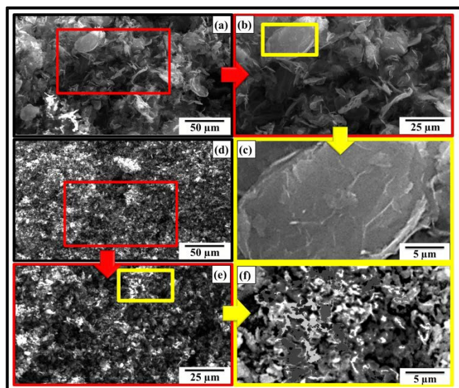
Fig. 1 SEM images: (a,b,c) MLG, and (d,e,f) NSG.
