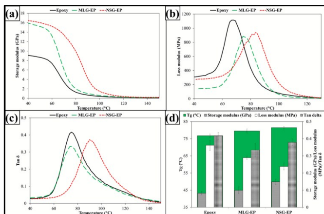
Fig. 5 Dynamic mechanical properties: (a) storage modulus, (b) loss modulus, (c) \text{Tan}\delta , and (d) T_g , and values of storage modulus, loss modulus and \text{Tan}\delta at T_g .
