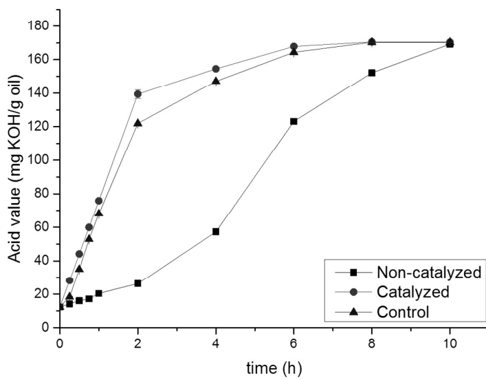
Figure 3. Acid value-time profile of Cu-catalyzed and non-catalyzed waste cooking oil hydrolysis reactions with respect to control system (dilute \text{H}_2\text{SO}_4 , pH 5.0) at 225^\circ\text{C} (water to acylglycerides molar ratio = 30:1)
