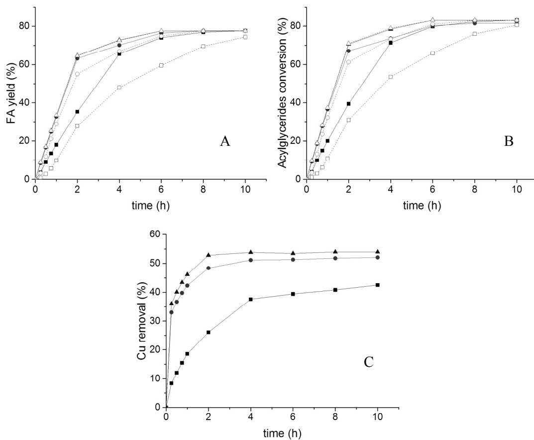
Figure 1. Percentage of (A) FA yield, (B) acylglycerides conversion, and (C) copper removal of hydrolysis reaction at (■) 200°C, (●) 225°C, and (▲) 250°C with control experiment points in open symbols (water to acylglycerides molar ratio of 30:1 and \text{CuSO}_4 concentration of 500 mg/kg)
