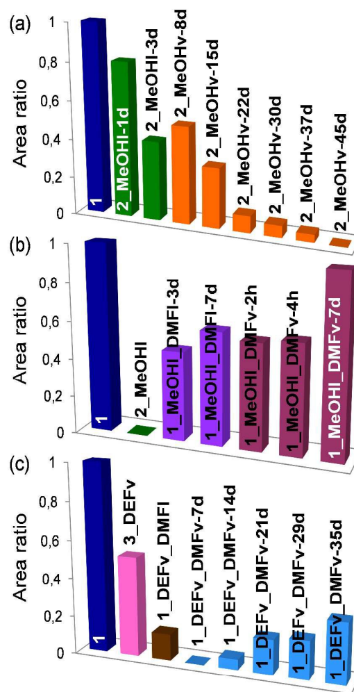
Fig. 7 Area ratios calculated with FTIR data using Eq. 1. (a) Exchange of DMF by MeOH (l and v) over time. Framework recovery using DMF (l and v) after exchange of (b) liquid MeOH and (c) vapour DEF.
