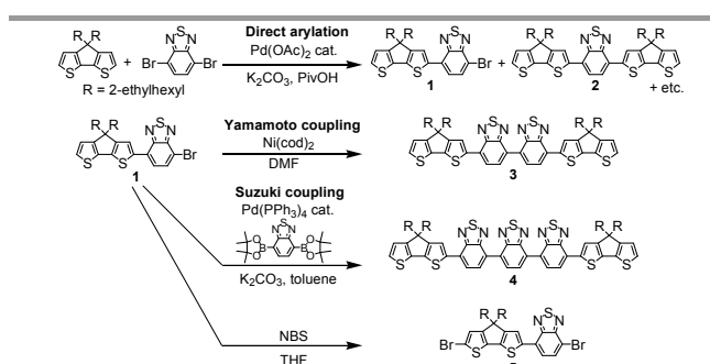
Scheme 1. Synthesis of monomers
