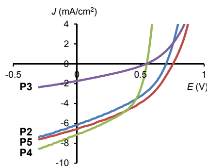
Fig. 5 Current density–Voltage characteristics of P2-P5 blended with PC 61 BM, measured under AM1.5G illumination.
