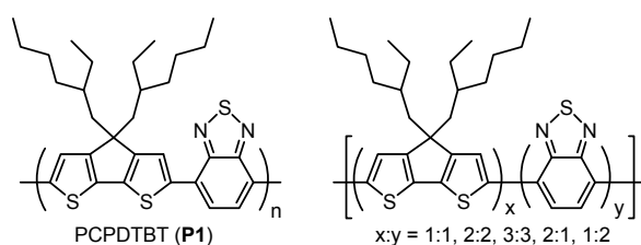
Fig. 1 PCPDTBT with permutations of repeating unit length and ratios
