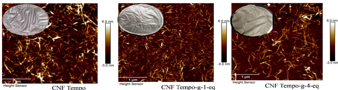
Figure 5. AFM Pictures of CNF Tempo, CNF Tempo-g-1-eq and CNF Tempo-g-4eq with films after grafting on the surface of cellulose (conc 0.1 %, tapping mode in air, area 3.3 X 3.3 μm²)
