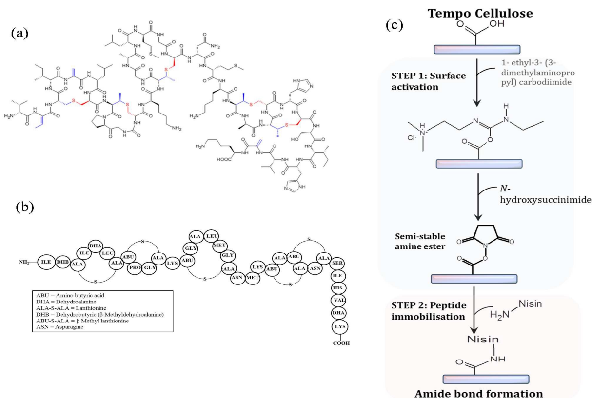
Figure 3 (a) Chemical structure of the lantibiotic Nisin Z (b) Primary structure of Nisin Z (Nisin Z contain asparagine instead of Histidine at position 27) (c) Schematic illustration of the main steps involved in the grafting of peptide Nisin Z on the surface of tempo cellulose.
