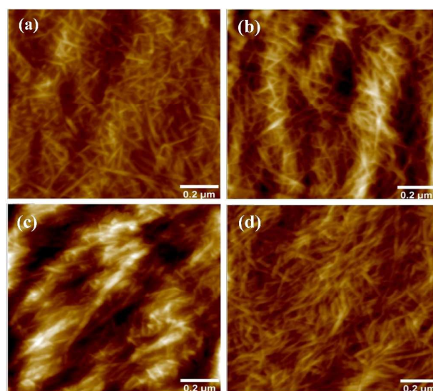
Figure 2. AFM standard tapping mode height sensor images in air of quartz gold sensors after each deposition cycle (a) nanocellulose (b) nanocellulose -Peptide nisin (c) nanocellulose -EDC/NHS (d) nanocellulose -EDC/NHS-nisin. z ranges from -19 to 20.6 nm.
