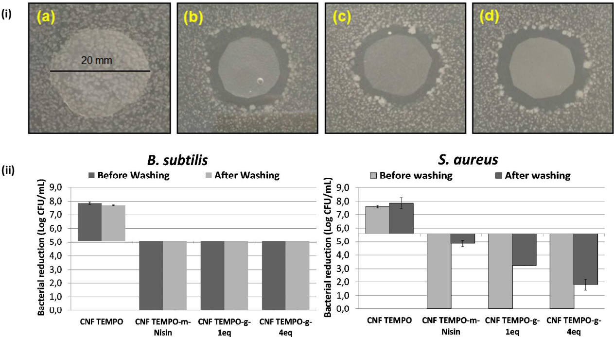
Figure 7. (i) Qualitative analysis of grafting on antimicrobial activity of B. subtilis : (a) CNF Tempo (b) CNF Tempo-m-Nisin (c) CNF Tempo-g-1eq (d) CNF Tempo-g-4eq, (ii) Effect of nisin on antimicrobial activity of Bacillus subtilis and Staphylococcus aureus on CNF Tempo, CNF Tempo-m-Nisin, CNF Tempo-g-1eq, and CNF Tempo-g-4eq.
