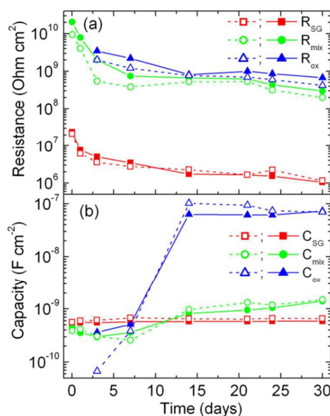
Fig. 7. Equivalent circuit parameters: resistance (a) and capacity (b) vs. time of immersion in 3% NaCl for ZE_Anod_SG (dashed lines, hollow marks) and ZE_Anod_Tr_SG (solid lines, filled marks).
