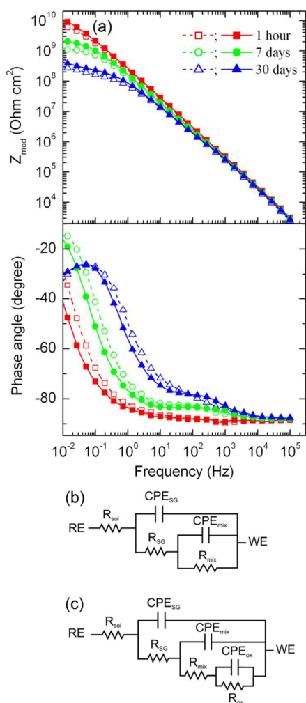
Fig. 6. Evolution of Bode plots (a) for ZE_Anod_SG (dashed lines, hollow marks) and ZE_Anod_Tr_SG (solid lines, filled marks) samples in 3% NaCl; equivalent circuits used for fitting experimental EIS spectra at different immersion times (b,c).
