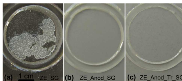
Fig.5. Optical photographs of ZE SG after 7 days (a) and ZE Anod_SG (b), ZE Anod_Tr_SG (c) samples after 30 days of immersion in 3% NaCl solution. The area exposed to the immersion test is 3.3 \text{ cm}^2 .
