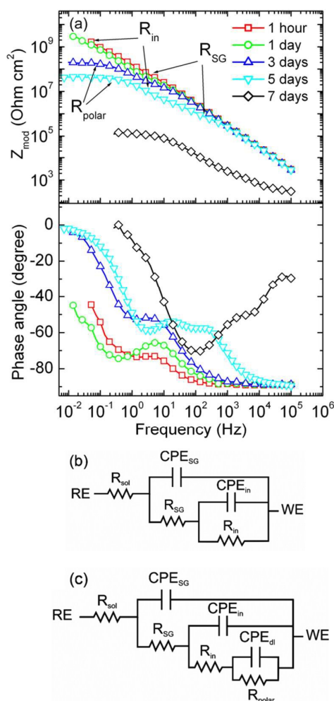
Fig.3 Evolution of Bode plots for ZE SG sample in 3% NaCl (a) and equivalent circuits used for fitting experimental EIS spectra at different immersion times (b,c).
