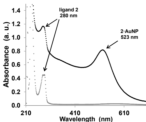
Fig. 1 UV-visible absorption spectra of free ligand 2 (grey) and in CH 2 Cl 2 (black). The peaks corresponding to the SPR band (523 nm) and the imidazolium ligand (280 nm) are visible in the 2 -AuNP spectrum.
