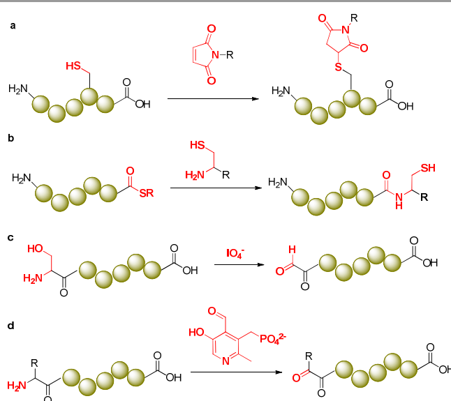
Figure 1. Typical bioorthogonal reactions utilizing native amino acid residues for protein modifications.
