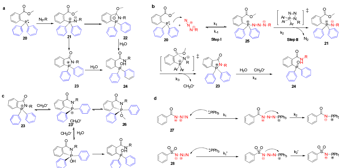
Figure 6. Mechanism and kinetic study of traceless-Staudinger reaction.
