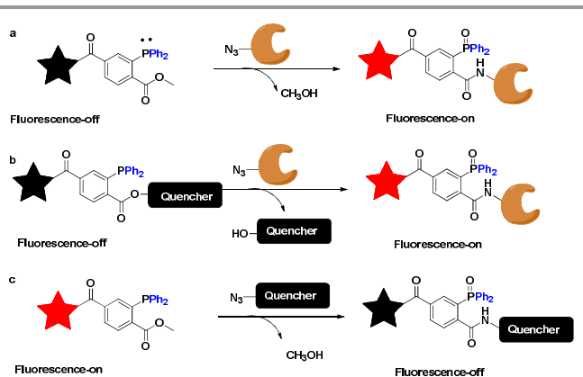
Figure 12. The application of traceless-Staudinger reaction for turn-on fluorescence labeling.
