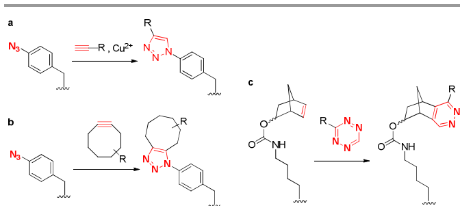
Figure 2. Three types of nCAA-based bioorthogonal reactions.
