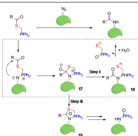
Figure 5. The possible side reaction of traceless-Staudinger reaction.
