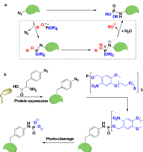
Figure 7. The Staudinger-Phosphite reaction.
