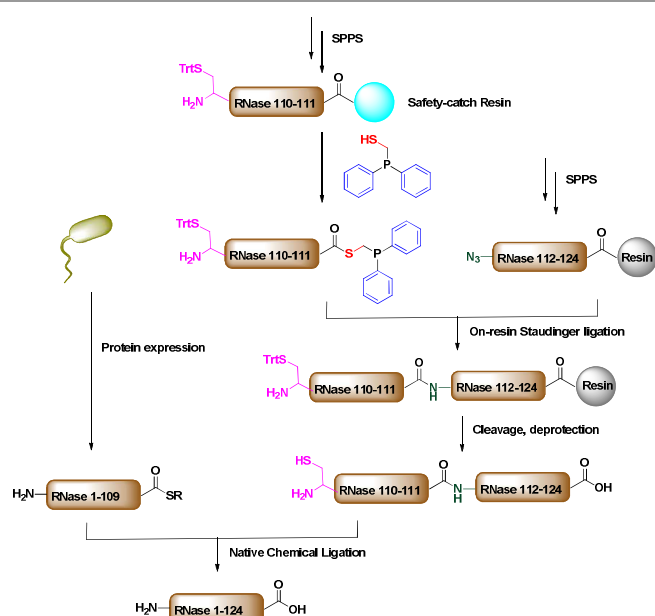
Figure 9. The applications of traceless-Staudinger reaction in vitro .
