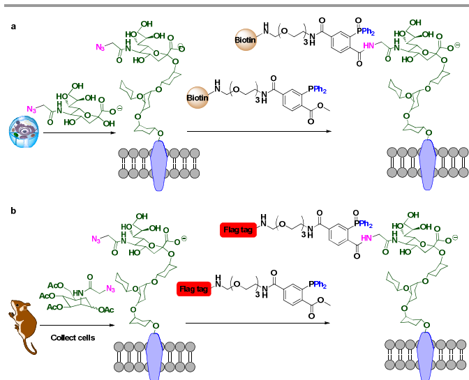
Figure 11. The applications of traceless-Staudinger reaction in living cells / in vivo .
