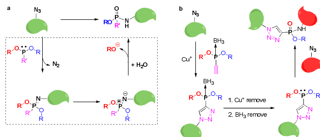
Figure 8. The Staudinger-Phosphonite reaction.
