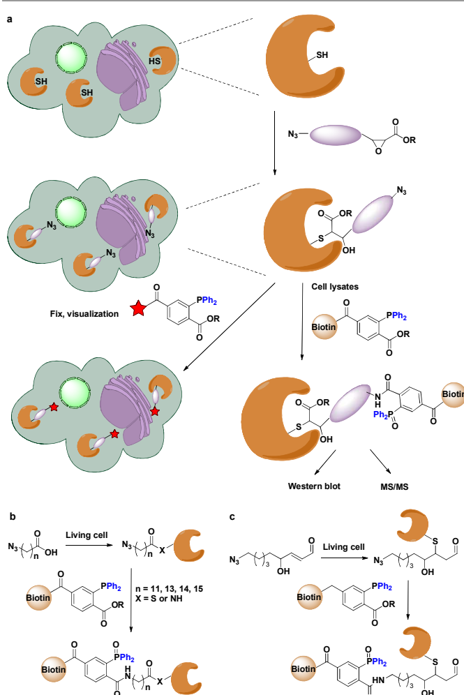
Figure 10. The applications of traceless-Staudinger reaction in cell lysate related systems.
