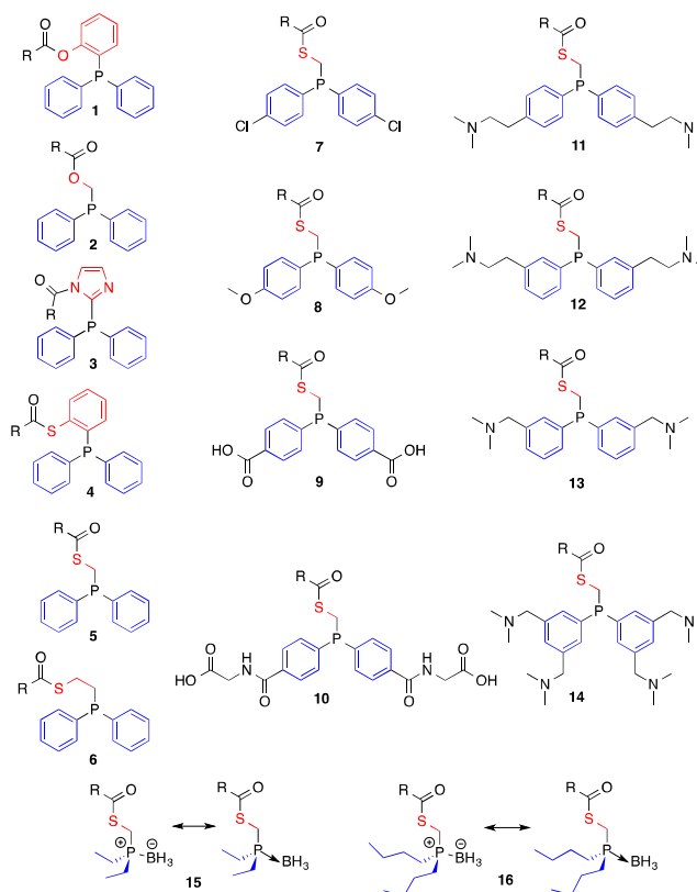
Figure 4. Chemical structures of different phosphine reagents for traceless-Staudinger reaction.
