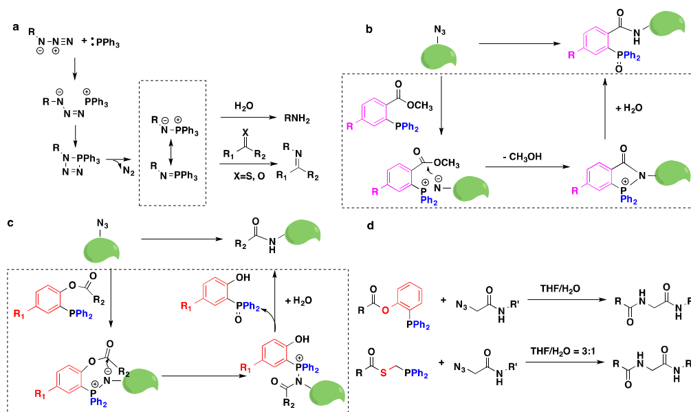
Figure 3. The mechanism and development of traceless-Staudinger reaction.
