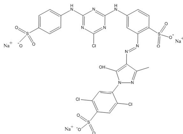
Figure 1. Molecular structure of Cibacron Brilliant Yellow 3G-P dye. Molecular weight = 872.97 g/mol.
