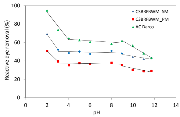
Figure 3. Evolution of reactive dye removal as a function of pH.
