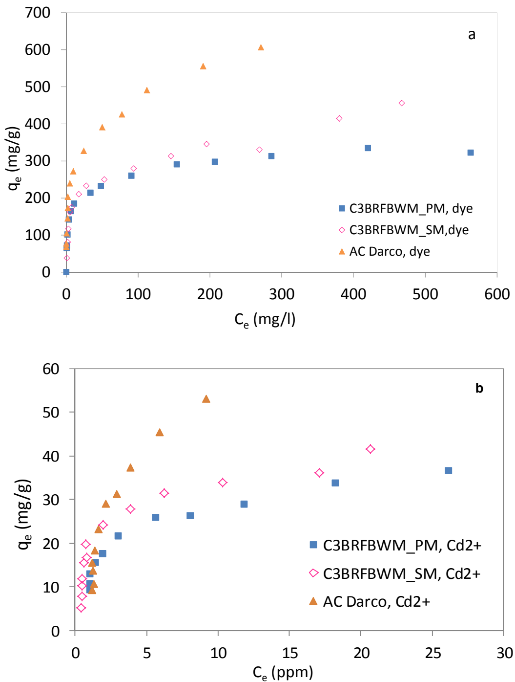
Figure 7. Adsorption isotherms of reactive dye (a) and Cd^{2+} (b) of the mixture dye+ Cd^{2+} solution on C3BRFBWM_PM, C3BRFBWM_SM and Darco KB-KJ
