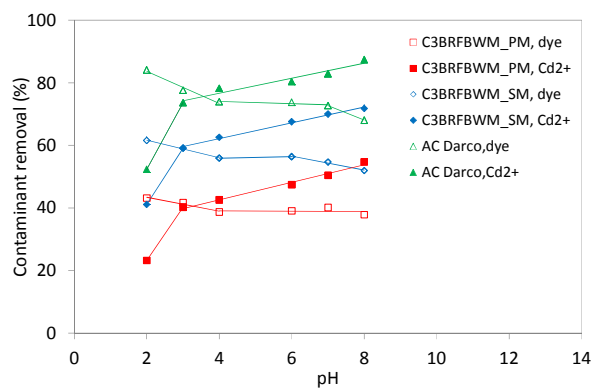
Figure 4. Variation in reactive dye + Cd 2+ removal as a function of pH.
