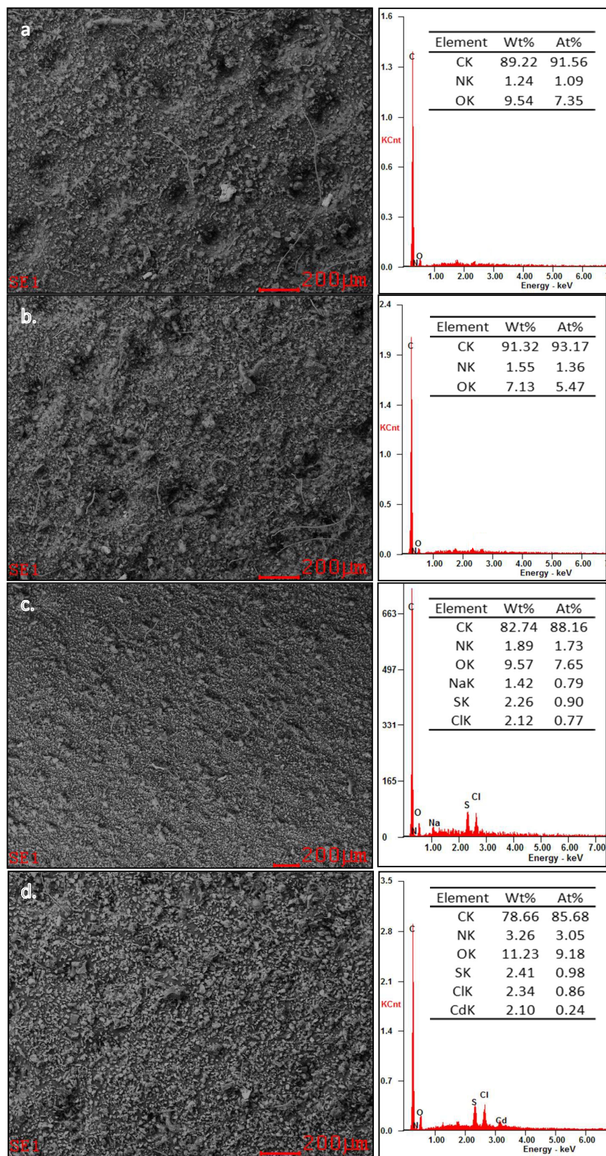
Figure 2. SEM-EDX results. a. before adsorption, b. after the adsorption of \text{Cd}^{2+} , c. after the adsorption of dye and d. after the adsorption of dye + \text{Cd}^{2+} .
