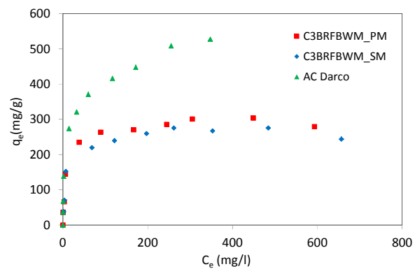
Figure 5. Adsorption isotherms for Cibacron Brilliant Yellow 3G-P dye by C3BRFBWM_PM, C3BRFBWM_SM and Darco KB-KJ.
