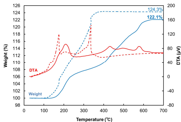
Figure 2. TGA (blue)-DTA (red) curves of BDVE-stabilized Cu fine particles (dashed line) and Cu pellet pressed at 100 °C (solid line). The pellet was pulverized into powder before the measurement.
