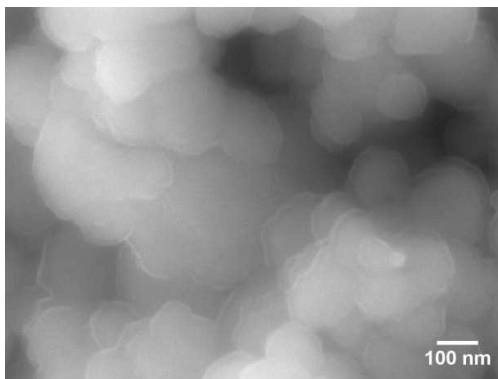
Figure 5 SEM image of the fracture surface of a Cu fine particle pellet pressed at 100 °C. Cu fine particles are covered by BDVE polymer residues.
