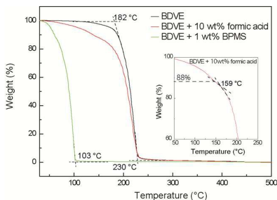
Figure 3. TGA charts of BDVE with and without acids. TG measurements were carried out under air flow ( 200 \text{ mL min}^{-1} ) at the heating rate of 1 \text{ }^\circ\text{C min}^{-1} . (black line) BDVE without acids. (red line) BDVE with 10 wt% of formic acid. (green line) BDVE with 1 wt% of BPMS. (Inset) Magnified curve of BDVE with 10 wt% of formic acid.
