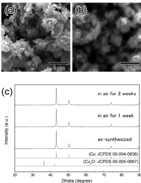
Figure 1. (a) A SEM image of as-synthesized BDVE (Poly-1,4-butanedioldivinylether)-stabilized Cu fine particles. (b) A SEM image of the particles produced on the large scale. (c) XRD patterns of BDVE-stabilized Cu fine particles. The sample was stored in air for 2 weeks.
