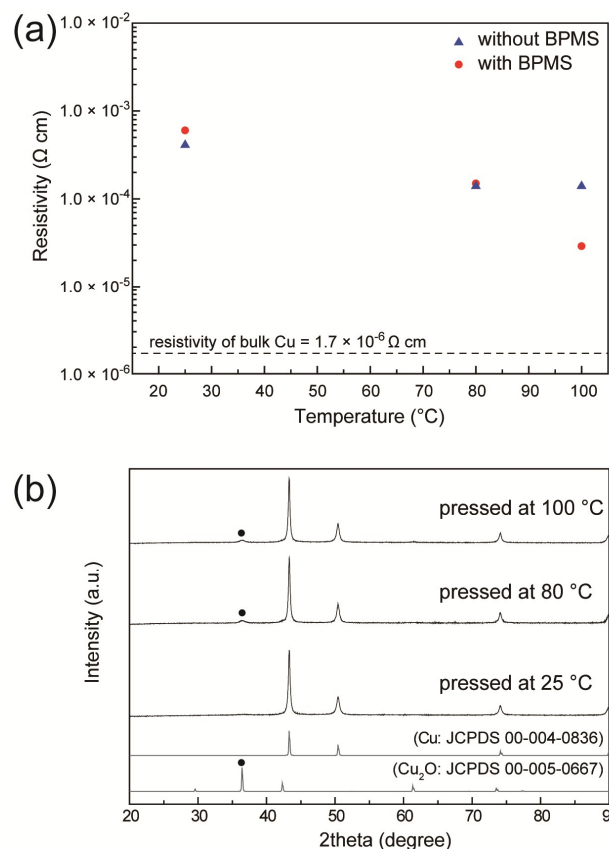
Figure 4. (a) Resistivities of hot-pressed Cu pellets with (circles: ●) and without (triangles: ▲) BPMS as the thermal acid generator. The resistivity of bulk copper is 1.7 \times 10^{-6} \text{ } \Omega \text{ cm} and is displayed as the dashed line. (b) XRD patterns of hot-pressed Cu pellets with BPMS. The (111) plane of \text{Cu}_2\text{O} is marked as closed circle (●).
