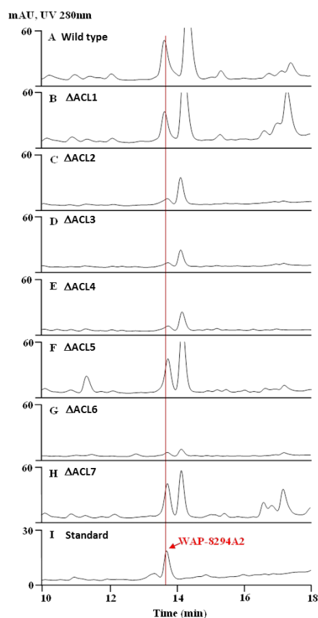
Fig. 2 HPLC analysis of metabolites from various strains of Lysobacter enzymogenes OH11. A: OH11 wild type; B-H: disruption mutants of ACL1 through ACL7, respectively; I: WAP-8294A2 standard. The detection wavelength was 280 nm.
