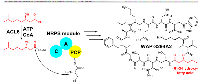
Fig. 6 Proposed mechanism for fatty acid incorporation in WAP-8294A2 biosynthesis. The fatty acid, ( R )-3-hydroxy-7-methyloctanoic acid, is activated by ACL6, and the resultant acyl-CoA is then recognized by the condensation (C) domain of the NRPS, which catalyzes the amide bond formation between the PCP-bound L-serine and the fatty acyl-CoA.
