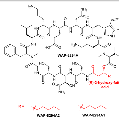
Fig. 1 Structure of the two main members of the WAP-8294A family.
