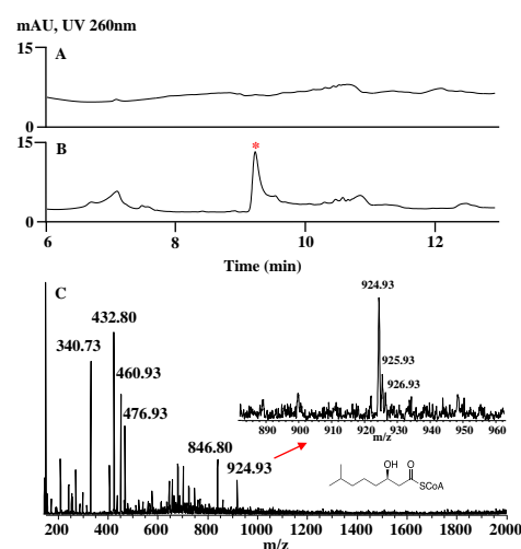
Fig. 5 HPLC and MS analysis of in vitro reaction products of ACL6 incubated with 3-hydroxy-7-methyloctanoic acid, ATP, and CoA. The ESI-MS signals were measured in positive single ion mode. A: HPLC of control reaction (without enzyme); B: HPLC of reaction with ACL6; C: ESI-MS of the peak from B.
