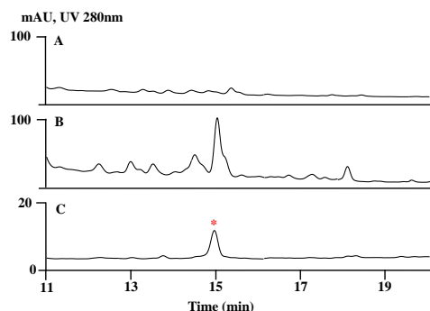
Fig. 3 HPLC analysis of metabolites in strains of Lysoibacter enzymogenes OH11. A: ACL6 in-frame deletion mutant; B: The ACL6 mutant supplemented with ( R )-3-hydroxy-7-methyloctanoic acyl-SNAC; C: WAP-8294A2 standard.
