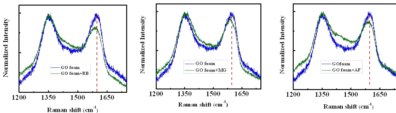
Figure 7. Raman spectra of GO foam before and after adsorption of RB, MG and AF dyes.
