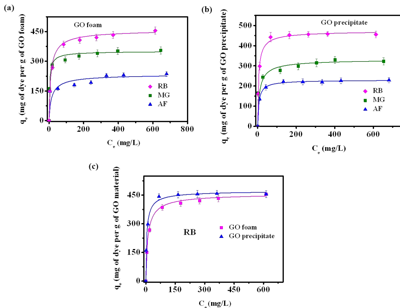
Figure 4. Adsorption isotherms and the corresponding fitting plots of RB, MG and AF dye molecules on (a) GO foam, and (b) GO precipitate at 37° C and natural pH (~3). Concentration of GO foam is 0.3 g/L and adsorption time is 8 h. (c) Comparison plot of adsorption isotherms of RB dye on GO foam and GO precipitate.
