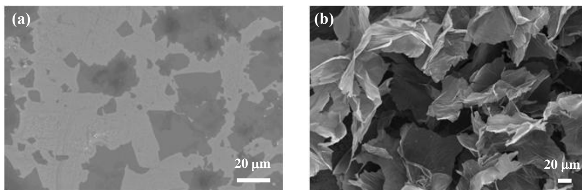
Figure 1. FE-SEM images of (a) GO flake and (b) GO foam of 1 wt %.
