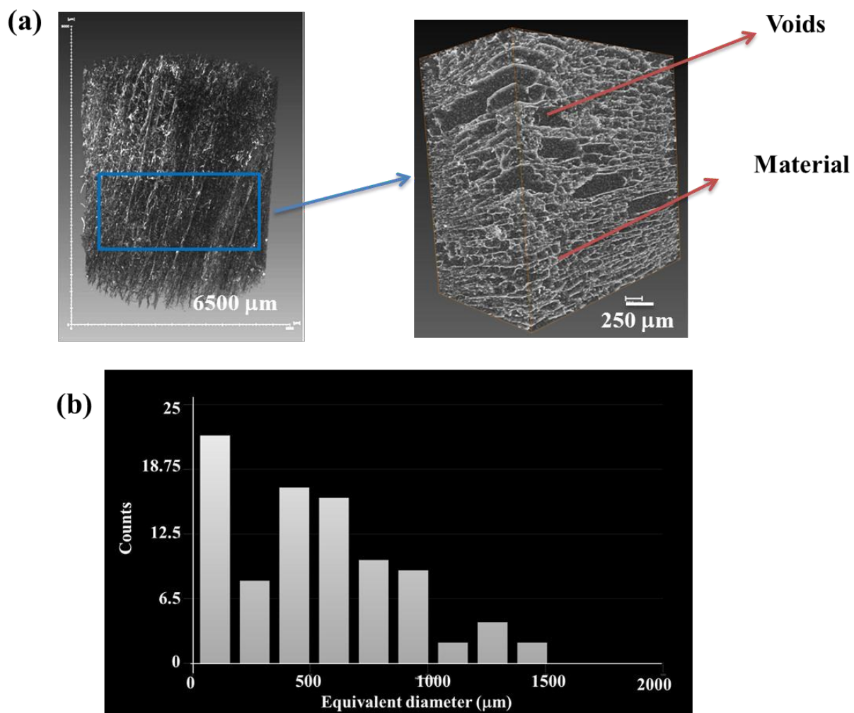
Figure 3. (a) 3D binary images of GO foam and the portion of the foam considered for the pore diameter analysis, (b) Histogram showing the distribution of equivalent diameter of pores in GO foam.
