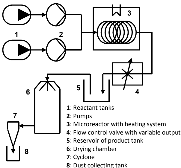
Fig 2. Design of the continuous-flow system coupled to spray dryer.
