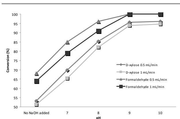
Fig 3. Effect of the pH of the L-cysteine solution adjusted with NaOH and the flow rate on the conversion of D-xylose and formaldehyde at 70°C.
