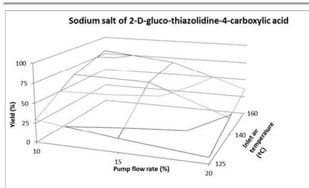
Fig 4. Powder recovery as a function of inlet air temperature and pump flow rate for the sodium salt of 2-D-gluco-thiazolidine-4-carboxylic acid.
