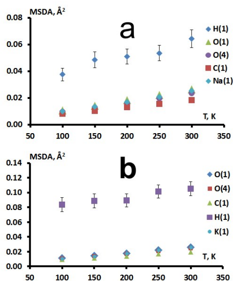
Fig. 6. Temperature dependence of mean-square displacement amplitudes (MSDA) of displacements for some heavy atoms ( U_{\text{eq}} values) and the H(1) atom involved in SSHB ( U_{\text{iso}} values) in 1 (a) and 2 (b).
