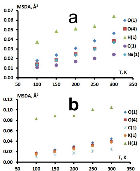
Fig. 5. Temperature dependence of mean-square displacement amplitudes (MSDA) of displacements for some heavy atoms (maximal \lambda_1 eigenvalues) and the H(1) atom involved in SSHB ( U_{\text{iso}} values) in 1 (a) and 2 (b).
