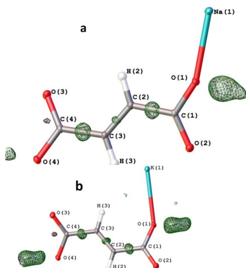
Fig. 4. Residual electron density maps for 1 (a) and 2 (b) plotted without the contribution of the H(1) atom by OLEX2 25 . Green surfaces denotes positive electron density at the \sim 0.32 \text{ e} \cdot \text{\AA}^{-3} level.
