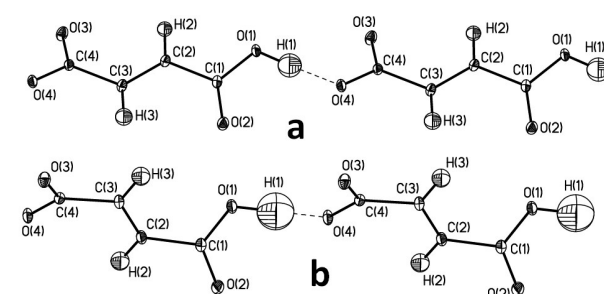
Fig. 3. Fragments of H-bonded anionic chains in crystals of 1 (a) and 2 (b). Atoms are represented by probability surfaces of atomic displacements ( p=50\% ): ellipsoids (non-hydrogen atoms) and spheres (hydrogen atoms).
