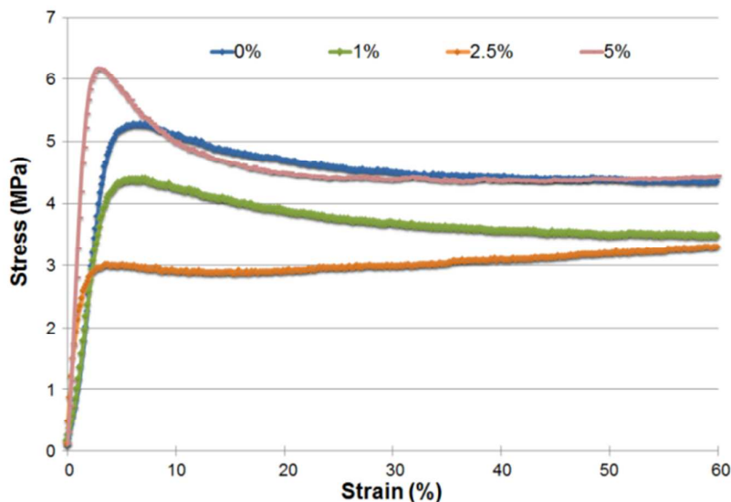
Figure 3. Typical stress-strain tensile curves of PCL-TIB/PLA 50 - b -PEG- b -PLA 50 blends (GABO Eplexor® 1500 N testing machine, 25 N cell force, 5 mm/min crosshead speed rate, 37°C). Percentages correspond to iodine weight ratios; samples were not loaded to failure.
