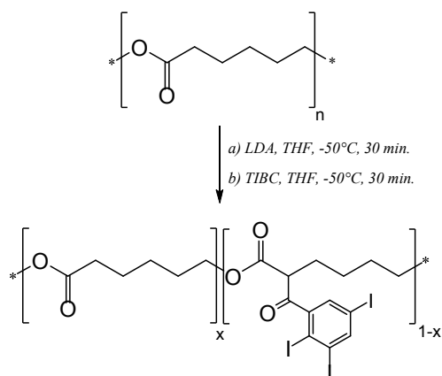
Scheme 1. Synthetic scheme for the preparation of poly(ε-caprolactone-co-α-triiodobenzoate-ε-caprolactone) (PCL-TIB)
