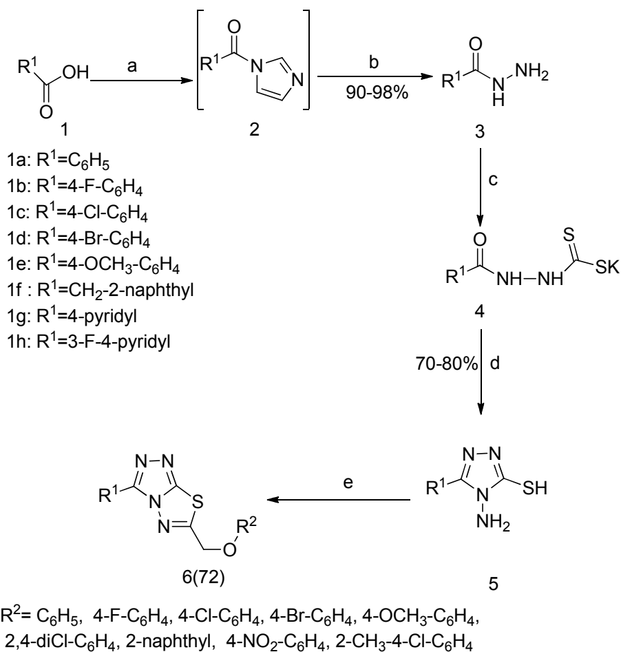
Scheme 1. Synthesis of 3,6-disubstituted triazolothiadiazoles. Reagents and conditions: (a) 1,1'-Carbonyldiimidazole, THF, 2 h, room temperature (rt); (b) N 2 H 4 H 2 O, rt, overnight; (c) CS 2 , KOH, EtOH, rt, 8 h; (d) N 2 H 4 H 2 O, rt, H 2 O, 2 h, rt/5 h, reflux; (e) ArOCH 2 CO 2 H, POCl 3 , MWI, 30 min, 155 °C.
