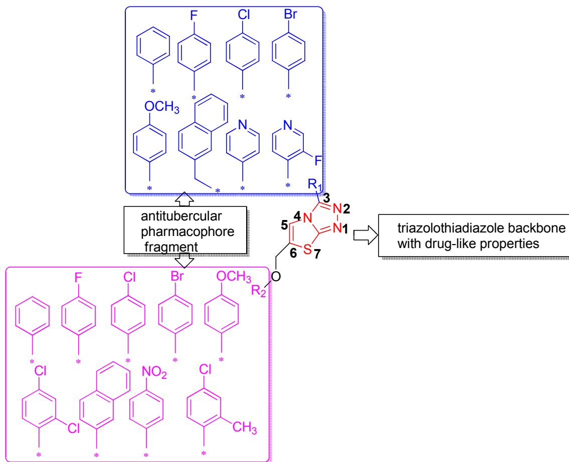
Fig. 2. Optimization of 3,6-disubstituted triazolothiadiazoles.
