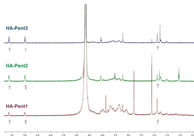
Fig. 2 1 H NMR spectra of HA-Pent derivatives recorded in D 2 O.
