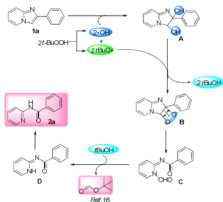
Scheme 3 Plausible mechanism of the direct transformation
