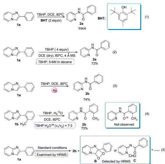
Scheme 2 Investigations of the mechanism
