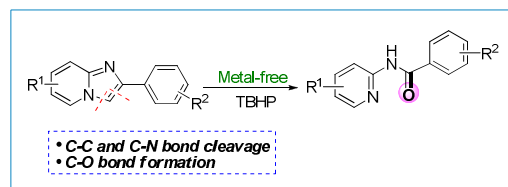
Scheme 1 Synthesis of N -(pyridin-2-yl)benzamides via C–C and C–N bond cleavage
