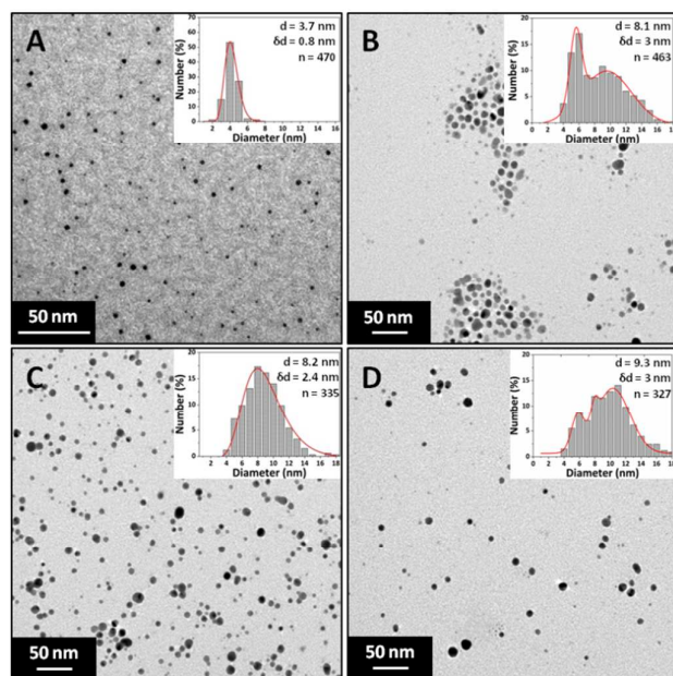
Fig 5: TEM images and particle size distributions of silver NPs synthesised at different silver nitrate concentrations. A: 0.05 mM, B: 0.15 mM, C: 0.25 mM and D: 0.4 mM. Concentration of trisodium citrate 0.5 mM, sodium borohydride 0.3 mM. Total flow rate 2.5 ml/min, 0.556 mm inner tube I.D.
