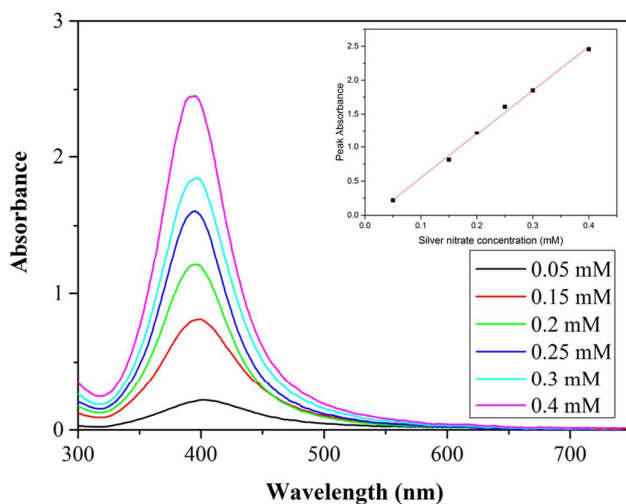
Fig 6: Absorbance peaks of silver NP synthesised at various silver nitrate concentrations in the range 0.05-0.4 mM. Total flow rate 2.5 ml/min, concentrations of trisodium citrate 0.5 mM, sodium borohydride 0.3 mM. 0.556 mm inner tube I.D. Inset: Silver nitrate concentration vs. peak absorbance for resonance peaks.
