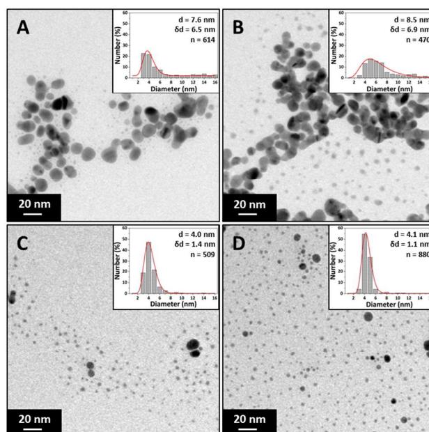
Fig 3: TEM images and particle size distributions of silver NPs synthesized at different trisodium citrate concentrations. A: 0.05 mM, B: 0.1 mM, C: 0.25 mM and D: 1.5 mM. Concentration of silver nitrate 0.1 mM, sodium borohydride 0.3 mM. Total flow rate 2.5 ml/min, 0.556 mm inner tube I.D.
