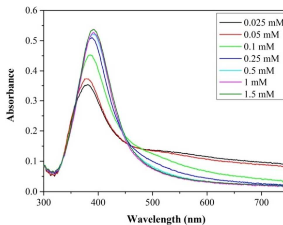
Fig 4: Absorbance peaks of silver NPs synthesised at various trisodium citrate concentrations in the range 0.025- 1.5 mM. Total flow rate 2.5 ml/min, concentration of silver nitrate 0.1 mM, sodium borohydride 0.3 mM. 0.556 mm inner tube I.D.
