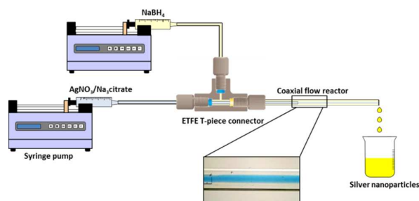
Fig 1: Schematic of the coaxial flow reactor setup. Insert shows flow visualization of laminar flow inside the coaxial flow reactor with blue dye flowing through the inner tube and water flowing through the outer tube.
