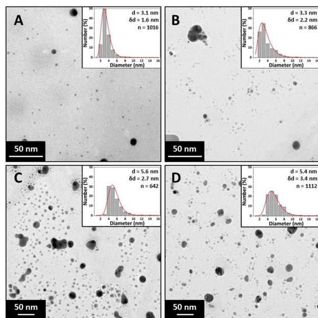
Fig 2: TEM images and particle size distributions of silver NPs synthesised at different total flowrates. A: 1 ml/min, B: 2.5 ml/min, C: 8 ml/min and D: 14 ml/min. Concentration of silver nitrate 0.2 mM, trisodium citrate 0.2 mM, sodium borohydride 0.6 mM. 0.798 mm inner tube I.D.
