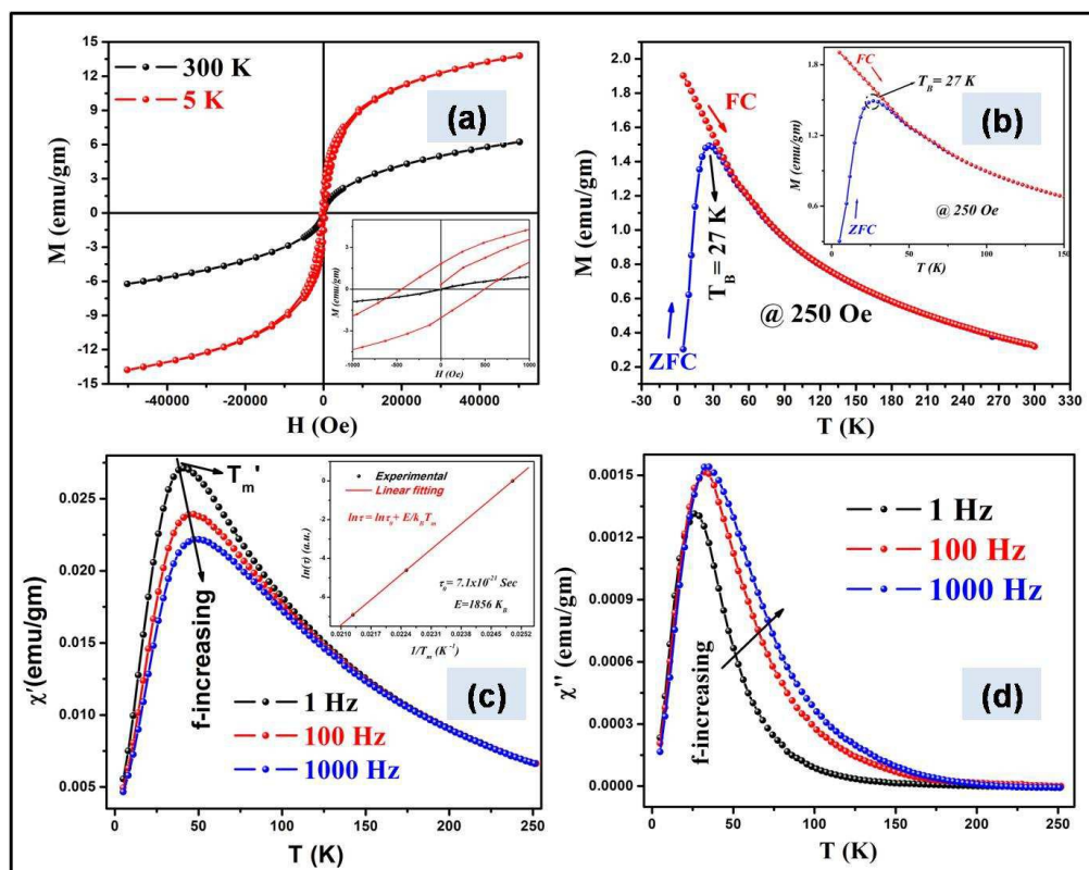
Fig. 6 (a) M-H curves of the composites measured at 300K and 5K (b) the M-T curves shows blocking below 27K and absence of dipolar interactions; (c) Real and (d) imaginary part of the susceptibility as a function of temperature measured at three different frequencies; (c) inset the Néel-Arrhenius plot showing superparamagnetic relaxation.
