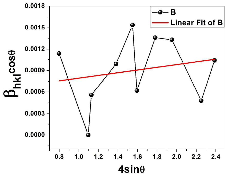
Fig. 2 Williamson-Hall Plot showing positive strain in the epsilon phase; the average crystallite size was equal to 250 nm.
