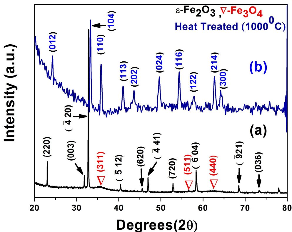
Fig. 1 Merged x-ray diffraction patterns of the (a) composite showing the formation of \epsilon -Fe 2 O 3 and Fe 3 O 4 phases; (b) the transformation to hematite upon heat treatment at 1000°C.
