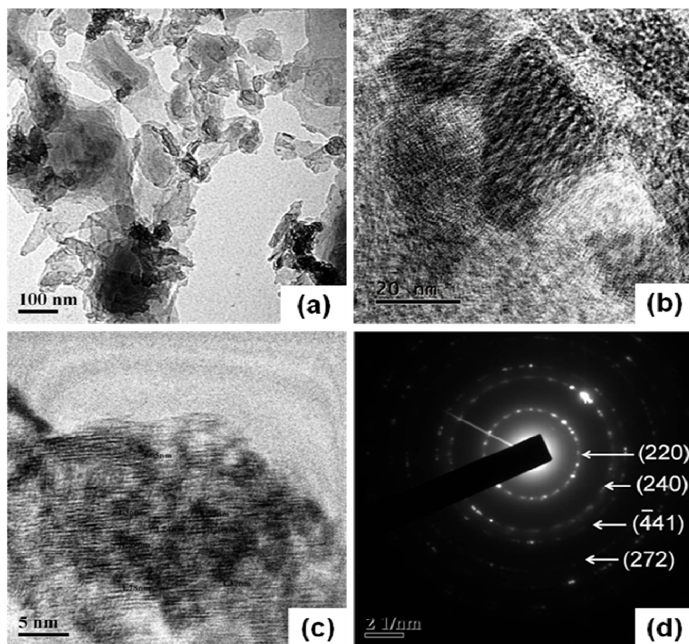
Fig. 3A (a-c) TEM micrographs showing G-IONP composites: (a) global picture of the composite flakes; (b) alignment of IONP particles on the flakes; (c) micro alignment of an enlarged flake (d) the indexed SAD pattern of (c) showing polycrystalline rings of the \epsilon - \text{Fe}_2\text{O}_3 phase.
