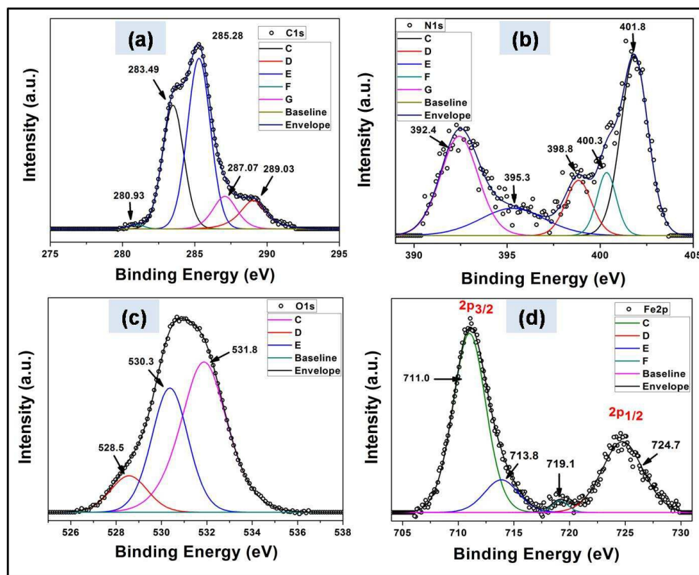
Fig. 5 XPS Spectra of the composite showing the spectral multiplets of (a) C1s , (b) N1s, (c) O1s and (d) Fe2p core level peaks.
