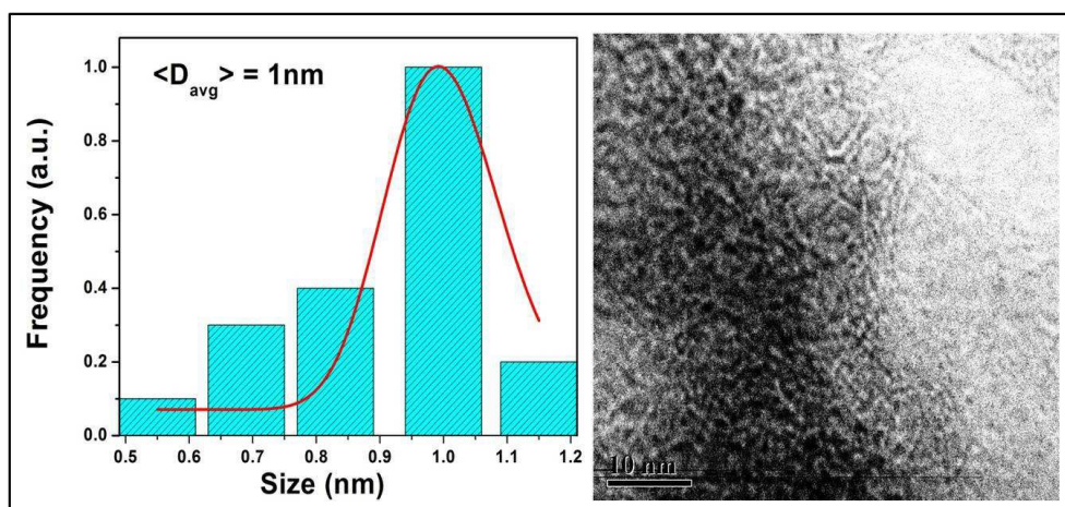
Fig. 3B Particle size distribution plot of uniformly distributed epsilon phase on graphene substrate with a mean particle size of 1 nm.
