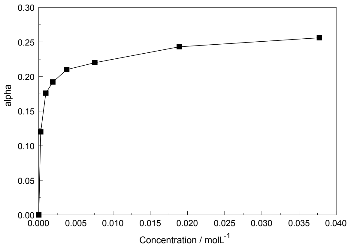
Figure 8. Degree of sulfato complex-formation, \alpha , as a function of the stoichiometric \text{La}_2(\text{SO}_4)_3 concentration at 23 °C.
