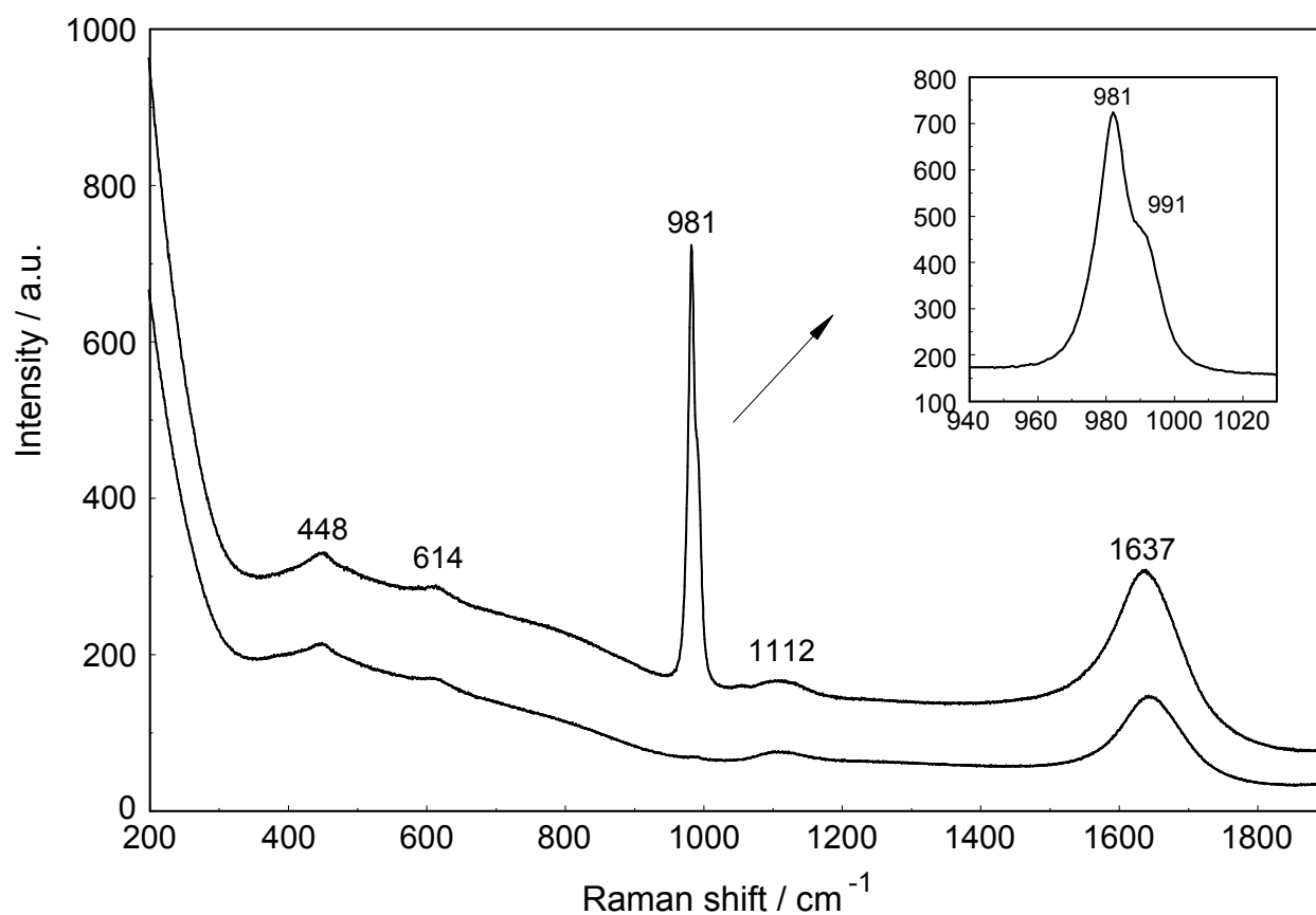
Figure 4. Raman scattering profiles (polarized and depolarized) of a 0.0376 \text{ molL}^{-1} \text{ La}_2(\text{SO}_4)_3 solution in the low wavenumber region from 200 - 1900 \text{ cm}^{-1} . In addition to the sulfate modes at 448, 614, 981 and 1112 \text{ cm}^{-1} the spectrum is dominated by the solvent with its two very broad librational bands at \sim 455 and \sim 720 \text{ cm}^{-1} of water and the deformation mode at 1637 \text{ cm}^{-1} ( I_{\text{pol}} scattering). Note that the \nu_1 \text{ SO}_4^{2-} stretching band, the strongest sulfate band is split into two component bands at 982 and 991 \text{ cm}^{-1} . Both \text{SO}_4^{2-} deformation modes at 451 and 614 \text{ cm}^{-1} appear on the broad librational band profile as weak bands. The \nu_3 \text{ SO}_4^{2-} antisymmetric stretching band at 1112 \text{ cm}^{-1} is also of weak intensity.
