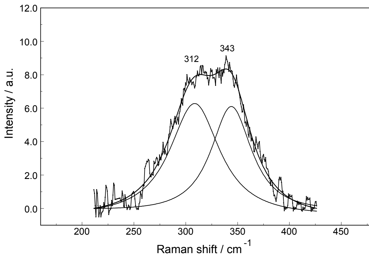
Figure 5. Band fit result on a difference Raman scattering profile (polarized scattering) of a 0.0376 molL -1 La 2 (SO 4 ) 3 solution from which the water background was subtracted. In addition to the difference Raman spectrum of the broad band feature, the sum curve of the fit and the two band components at 312 cm -1 and 343 cm -1 are shown.
