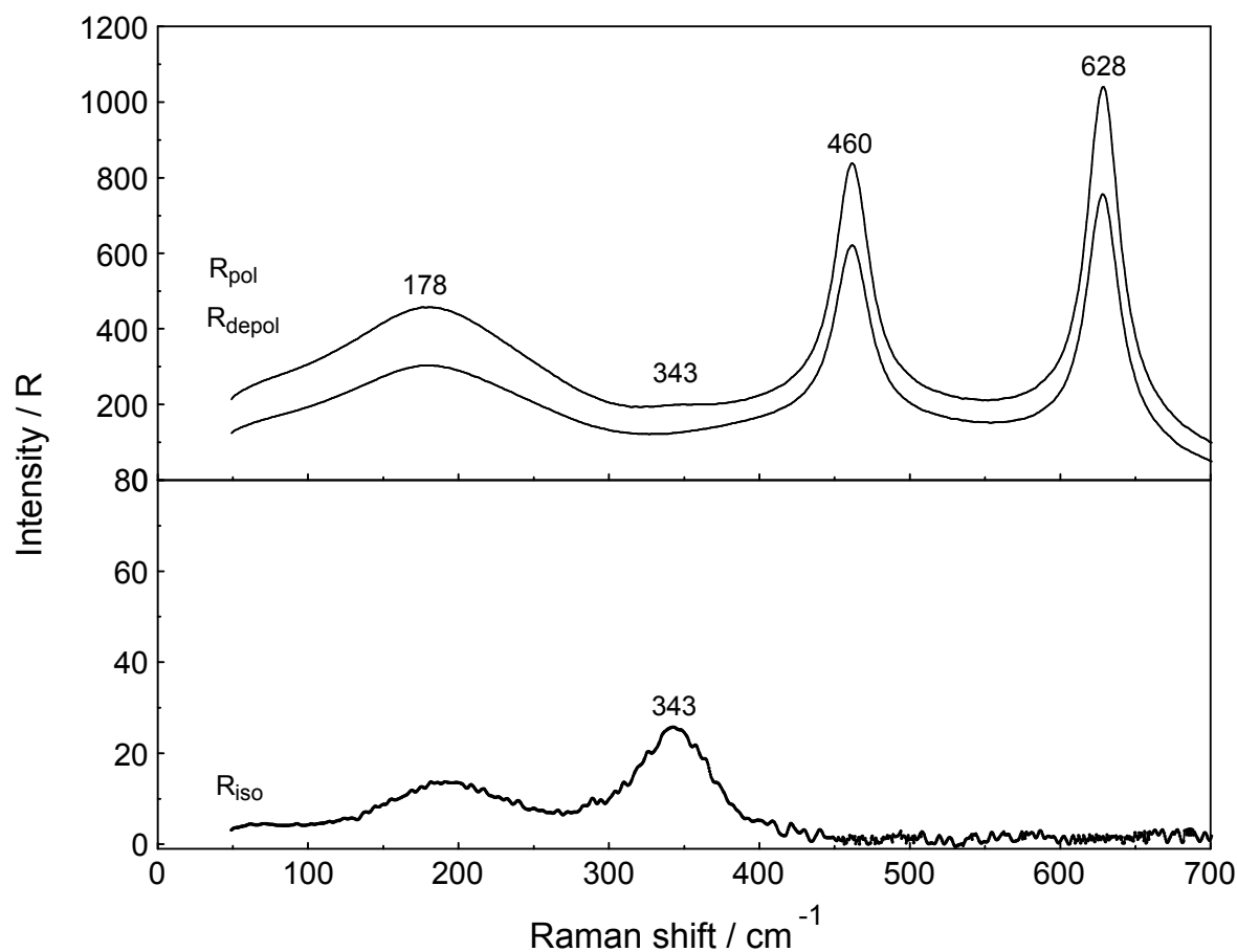
Figure 1. Raman scattering profiles of a 0.249 \text{ molL}^{-1} ( R_w = 214 ) \text{La}(\text{ClO}_4)_3(\text{aq}) . Upper panel: R_{\text{pol}} and R_{\text{depol}} scattering. Note the very weak band at 343 \text{ cm}^{-1} due to the symmetric breathing mode of [\text{La}(\text{OH}_2)_9]^{3+} . In addition, the deformation modes of \text{ClO}_4^-(\text{aq}) which dominate the spectrum at 460 \text{ cm}^{-1} and 628 \text{ cm}^{-1} are shown. The band at 178 \text{ cm}^{-1} ( R_{\text{VV}} ) is due to the restricted O-H \cdots O bonds of the water H-bond network. Lower panel: Isotropic scattering in R-format. Note the very weak band at 343 \text{ cm}^{-1} due to the symmetric breathing L-O mode. The isotropic mode at 182 \text{ cm}^{-1} is due to the restricted O-H \cdots O bonds of the water H-bond network.
