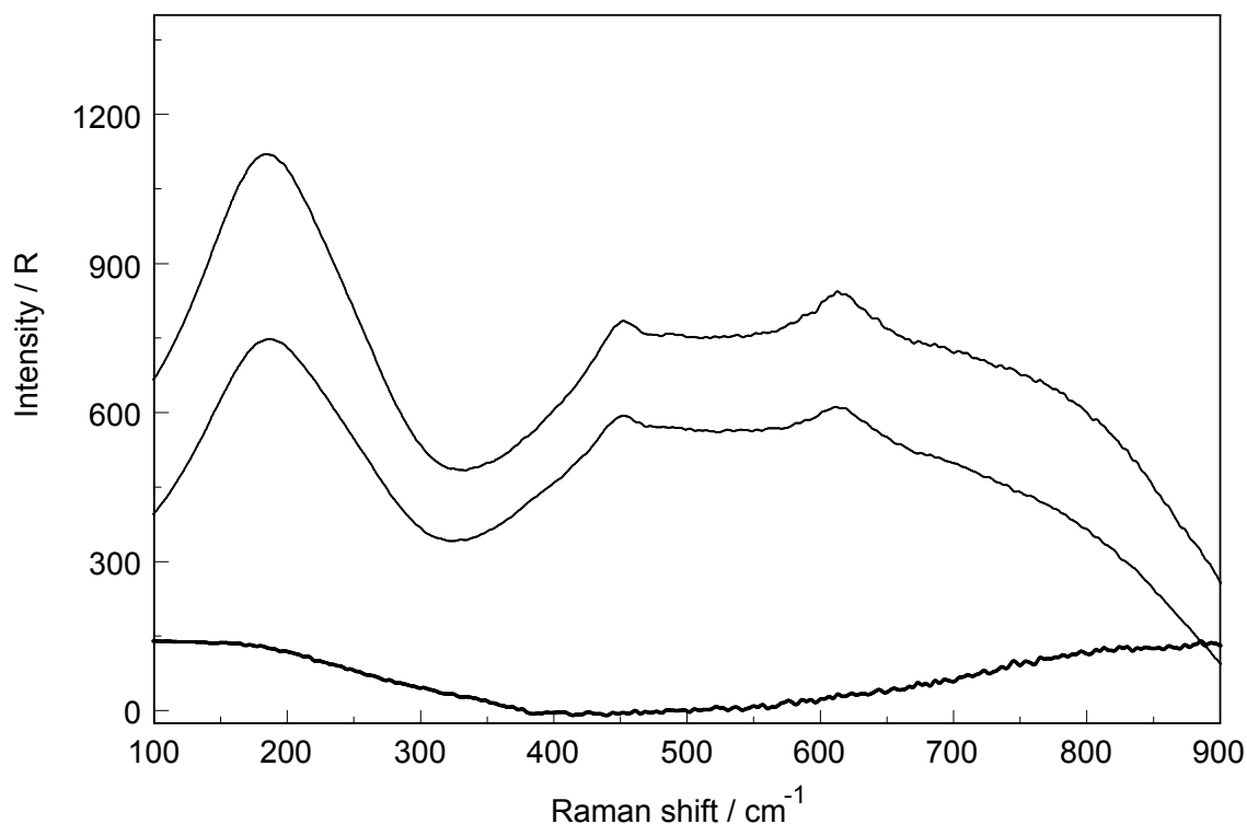
Figure 6A. Raman scattering profiles (polarized, depolarized and isotropic) of a 0.0376 \text{ molL}^{-1} \text{ La}_2(\text{SO}_4)_3 solution in the low wavenumber region from 100 - 900 \text{ cm}^{-1} . Shown are the restricted translation band \text{O-H}\cdots\text{O} at 181 \text{ cm}^{-1} and the very broad and dominating bands at ca. 455 and 720 \text{ cm}^{-1} due to the librational bands of \text{H}_2\text{O} . The two weak deformation modes of \text{SO}_4^{2-} at 448 and 614 \text{ cm}^{-1} are “sitting” on the broad librational band structure.
