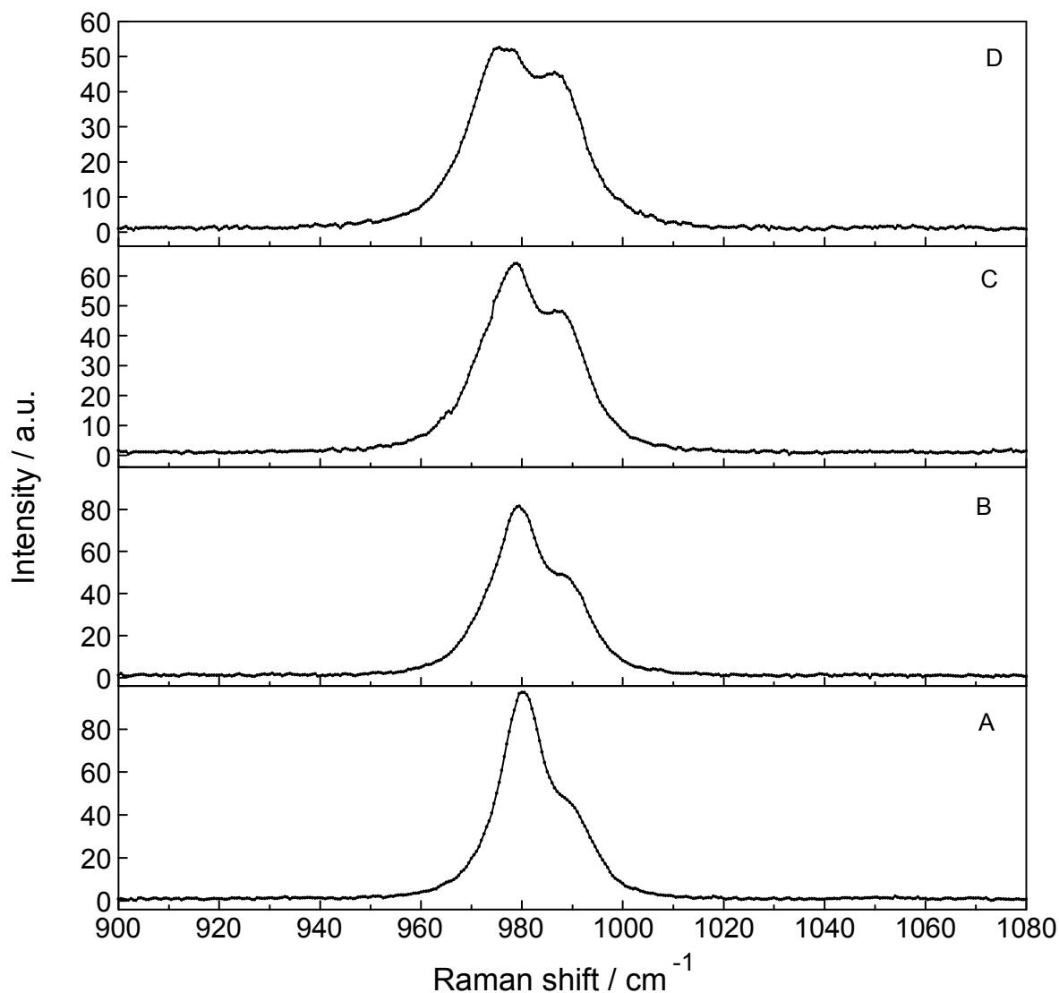
Figure 9. Temperature dependence of a series of isotropic Raman scattering profiles of a 0.0093 \text{ molL}^{-1} \text{La}_2(\text{SO}_4)_3 solution in the wavenumber range from 900 - 1080 \text{ cm}^{-1} ( \nu_1 \text{SO}_4^{2-} stretching region). From bottom to top: 24.0^\circ\text{C} , 50.0^\circ\text{C} , 75.0^\circ\text{C} and 98.0^\circ\text{C} . Note that with temperature increase the bands at 980.3 \text{ cm}^{-1} of “free” \text{SO}_4^{2-}(\text{aq}) and coordinated \text{SO}_4^{2-} at 991 \text{ cm}^{-1} shift slightly to lower wavenumbers. The intensity of the band at 980.5 \text{ cm}^{-1} of “free” \text{SO}_4^{2-}(\text{aq}) , however, decreases markedly with the rise in temperature while the intensity of band of the complex bound sulfate at 991 \text{ cm}^{-1} increases considerably. At 24^\circ\text{C} \sim 25\% of the sulfate occurs in the \text{La}^{3+} - sulfato complex species while at 98.0^\circ\text{C} \sim 42\% of the sulfate is bound as a sulfato-complex.
