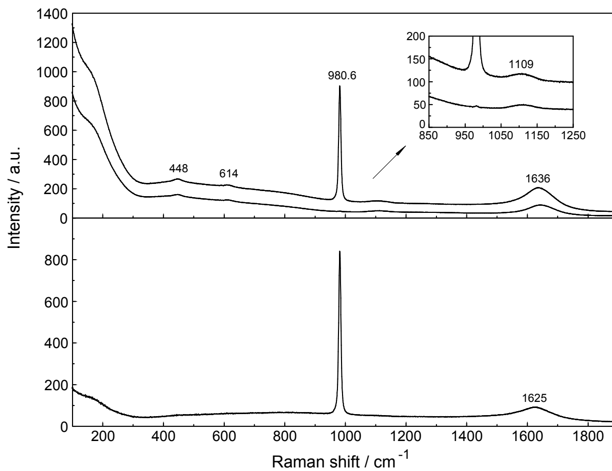
Figure 2. Overview Raman profiles of a 0.101 molL -1 Na 2 SO 4 solution. The I VV and I VH scattering orientations (upper panel) are given and in the lower panel the isotropic scattering.
