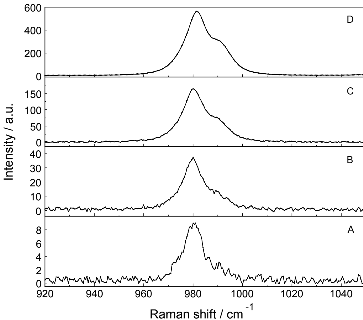
Figure 7. Dilution series of polarized Raman scattering profiles of selected \text{La}_2(\text{SO}_4)_3 solutions in the wavenumber range from 920 - 1060 \text{ cm}^{-1} ( \nu_1 \text{SO}_4^{2-} stretching region). From bottom to top: A) 0.000263 \text{ mol}\cdot\text{L}^{-1} , B) 0.00121 \text{ mol}\cdot\text{L}^{-1} , C) 0.00606 \text{ mol}\cdot\text{L}^{-1} and D) 0.0302 \text{ mol}\cdot\text{L}^{-1} \text{La}_2(\text{SO}_4)_3 solution. Note the split of the S-O stretching band into a band at 981.3 \text{ cm}^{-1} of “free” \text{SO}_4^{2-} and coordinated \text{SO}_4^{2-} at 991 \text{ cm}^{-1} as a separate band component.
