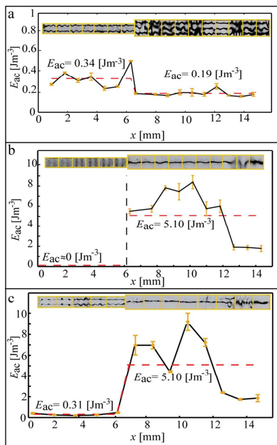
Figure 3: Measurements of the spatial distribution of the acoustic energy density in Zone 1 ( 0 \text{ mm} < x < 6 \text{ mm} ) and Zone 2 ( 6 \text{ mm} < x < 15 \text{ mm} ) when actuation one transducer at the time (a-b), or two transducers simultaneously (c). (a): Actuation of the pre-alignment transducer (Zone 1) at 4.45 MHz. (b): Actuation of the separation transducer (Zone 2) at 1.39 MHz. (c): Actuation of both the pre-alignment and separation transducers (Zone 1 and 2) transducer at 4.45 MHz and 1.39 MHz, respectively. The diagrams show the acoustic energy densities when selecting driving voltages for optimal separation performance. The standard deviations correspond to three repetitions of each experiment. The plotted energy densities are the components responsible for particle manipulation in the y direction (along the channel width), since the utilized method for measuring energy density is a one dimensional method. Error bars correspond to \pm 1\text{SD} from three repetitions of the experiment.
