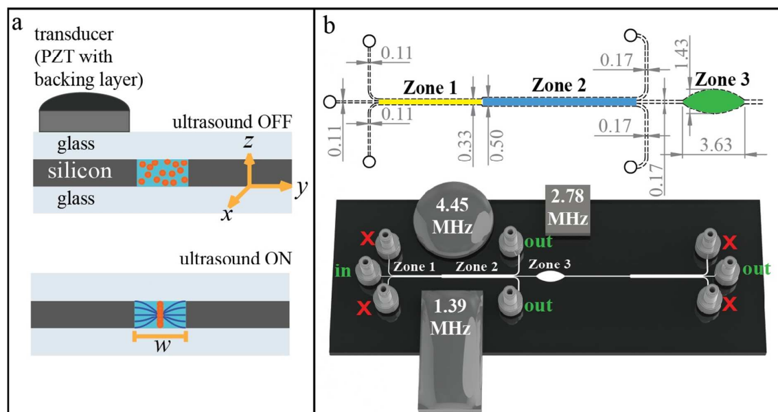
Figure 1. (a): Schematic cross-section view of the microchip device (not to scale). The chip consists of a silicon layer (dark gray) sandwiched in between of two glass layers (light gray). It is actuated by (b): three different ultrasound transducers, 4.45 MHz (Zone 1), 1.39 MHz (Zone 2), and 2.78 MHz (Zone 3). The frequencies are selected to generate two pressure nodes in Zone 1, one pressure node in Zone 2, and a multitude of pressure nodes in Zone 3. In the upper panel in (b), the channel dimensions are shown in gray (mm), and the different zones are marked in colors. Two of the transducers (1.39 MHz and 4.45 MHz) used backing layers, as illustrated in (a), while the 2.78 MHz transducer was air-backed. Two suction-mode syringe pumps were used: One connected to the two outlets between Zone 2 and Zone 3, and one connected to the outlet to the right, after Zone 3.
