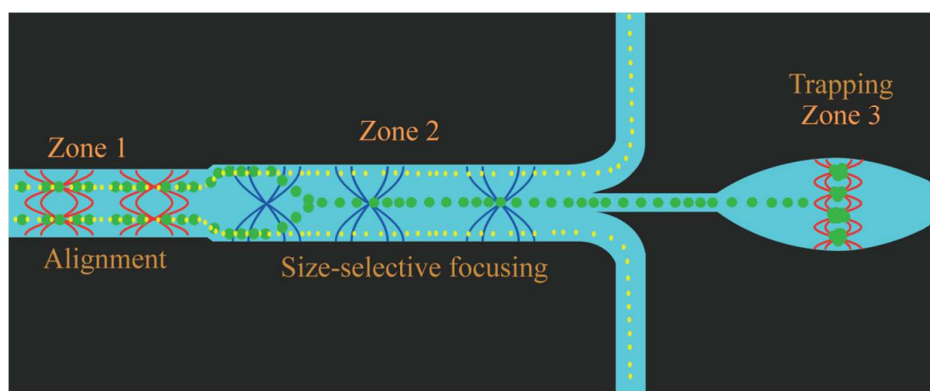
Figure 2: Conceptual illustration of the three-step acoustophoresis method. Cells or beads are pre-aligned into two acoustic pressure nodes in Zone 1 (4.45 MHz and 9 Vpp actuation), followed by size-based separation of larger cells or beads into one node in Zone 2 (1.39 MHz and 16 Vpp actuation), and finally isolation, retention and up-concentration of the larger cells or beads in Zone 3 (2.78 MHz and 10 Vpp actuation).
