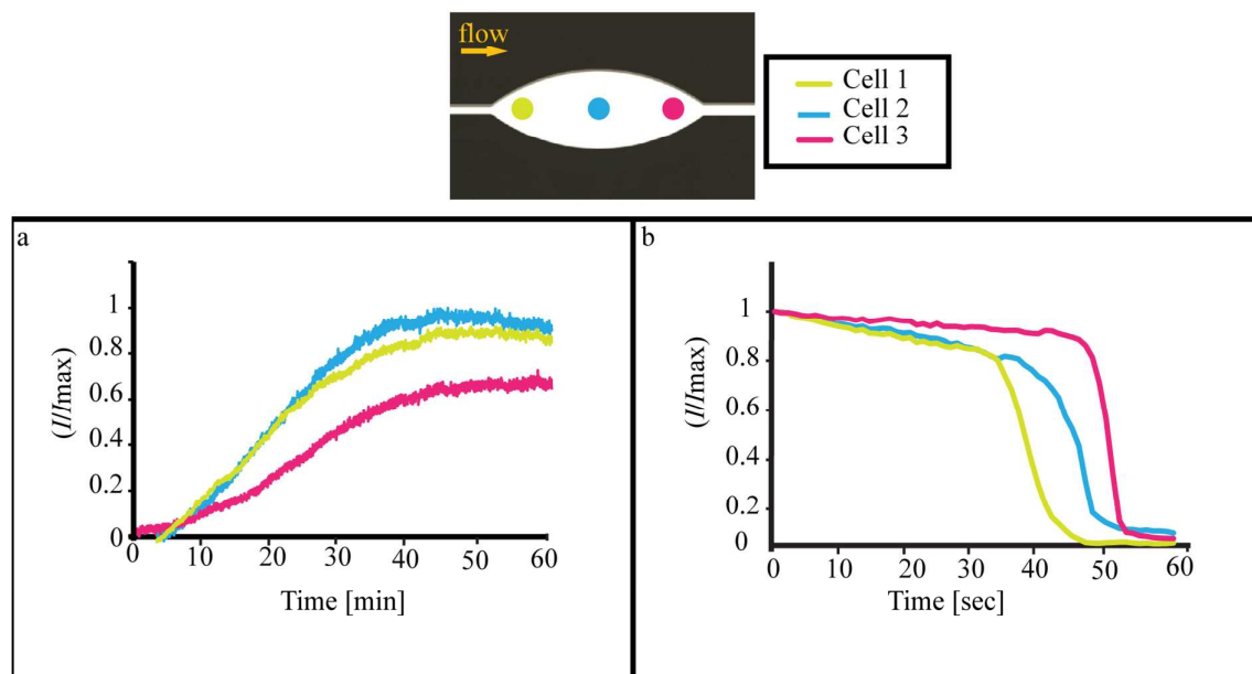
Figure 9: Quantification of the dynamics of uptake (a) and Saponin (1%)-induced release (b) of calcein-AM (5 \mu\text{M} ) in three individual A549 cells trapped in different parts of the trapping chamber (Zone 3). The flow rates are the same as in the separation and trapping experiments: 4.5 \mu\text{l}/\text{min} injected flow, out of which 0.5 \mu\text{l}/\text{min} is passing the trapping chamber (Zone 3).
