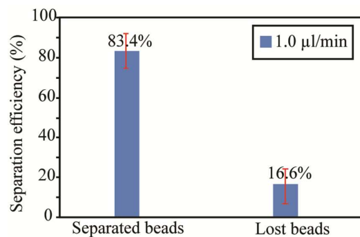
Figure 4: Separation efficiency of 10 \mu\text{m} polystyrene beads from 5 \mu\text{m} polystyrene beads when using 1.0 \mu\text{l}/\text{min} flow rate in the center channel after Zone 2, and 2.0 + 2.0 \mu\text{l}/\text{min} flow rates in the two side channels after Zone 2. The experiment was optimized for minimizing the number of 5 \mu\text{m} beads entering Zone 3. Error bars correspond to \pm 1\text{SD} from three repetitions of the experiment.
