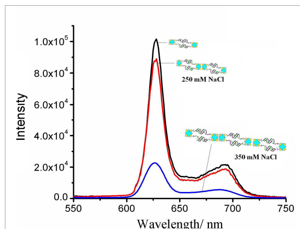
Fig.6 Emission spectra of PpIX, (ODN1) 2 -PpIX, (ODN1) 2 -PpIX-(ODN2) 2 -PpIX ( \lambda_{exc} = 400 nm). Number of nanocages depicted are symbolic to denote more aggregation at higher salt concentration.
