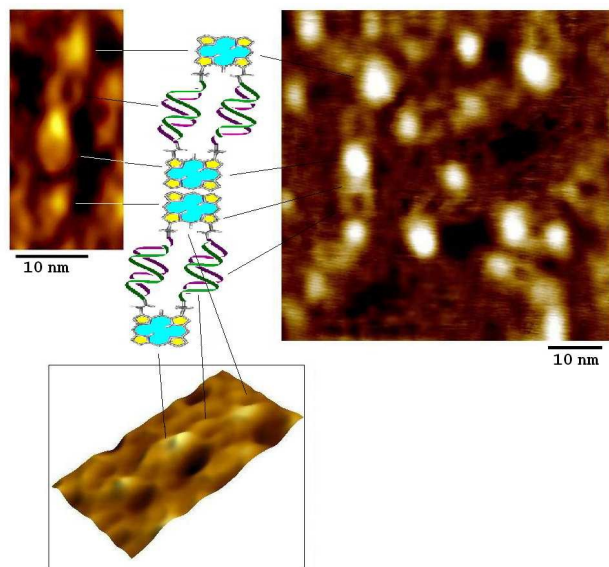
Fig.4 AFM image showing self assembled (ODN1) 2 -PpIX- (ODN2) 2 -PpIX leading to the formation of explicit 2D nanocages
