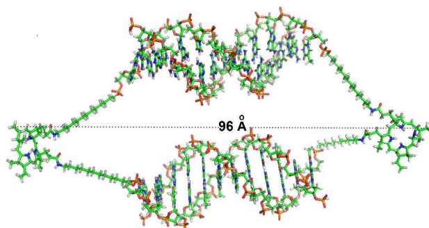
Fig.7 Computational studies depicting explicit nanocages formation. The structure of DNA and PpIX are represented in sticks with carbon, nitrogen, oxygen and phosphate atoms shown in green, blue, red and orange colors respectively using the PyMol molecular graphics system with head to tail length of 9.6 nm.
