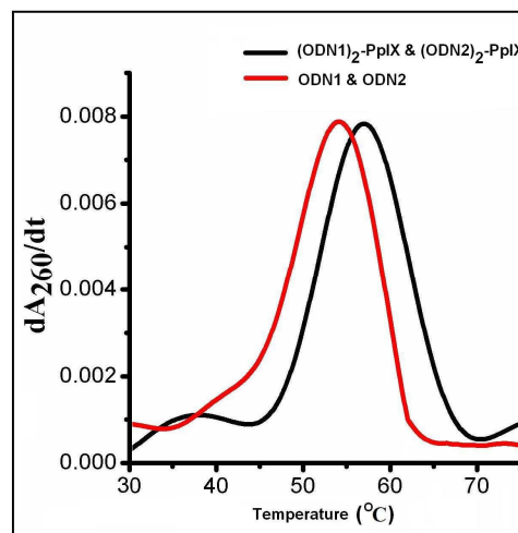
Fig.3 Thermal melting profile of normal ODN1-ODN2 and (\text{ODN1})_2\text{-PpIX}-(\text{ODN2})_2\text{-PpIX} .
