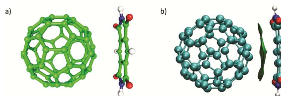
Fig 4. a) Optimized geometry of fullerene – PMDI complex. b) NCI visualization index of fullerene – PMDI complex. Green surface indicates the area of weak, attractive \pi – \pi interactions between two molecules.
