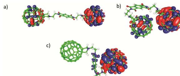
Fig 6 Electron density difference maps between first excited and ground state for a) extended, b) single folded and c) double folded conformer of compound 1a . The blue lobes represent area of higher electron densities in excited state than in the ground state. The red lobes represent area of lower electron densities in excited state than in the ground state.
