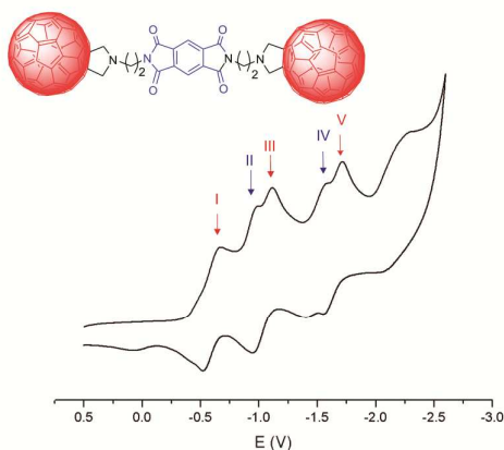
Fig 3 Cyclic voltammogram (CV) of 2a at 50 mV s -1 rate in o -dichlorobenzene:DMF = 2:1 mixture, containing 0.1M n Bu 4 NPF 6 .
