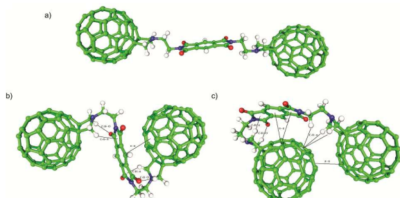
Fig 5. Mapping non-covalent intermolecular interactions in 2a .
