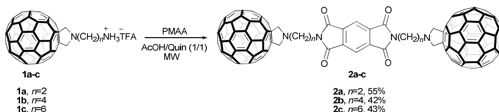
Scheme 1. Synthesis of C_{60} -PMDI- C_{60} molecular dumbbells 2a-c
