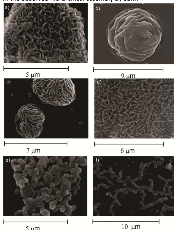
Fig 8. SEM images of 2a prepared from a) toluene/dioxane, b) toluene/ Pr -OH; 2b prepared from c) toluene/dioxane, d) toluene/ Pr -OH and 2c prepared from e) CHCl_3 / Pr -OH, f) CHCl_3 /dioxane.
