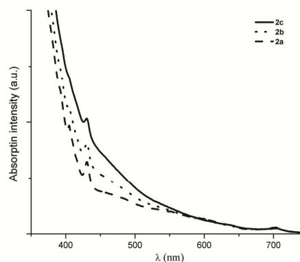
Fig 2. UV-Vis spectra of compounds 2a-c
