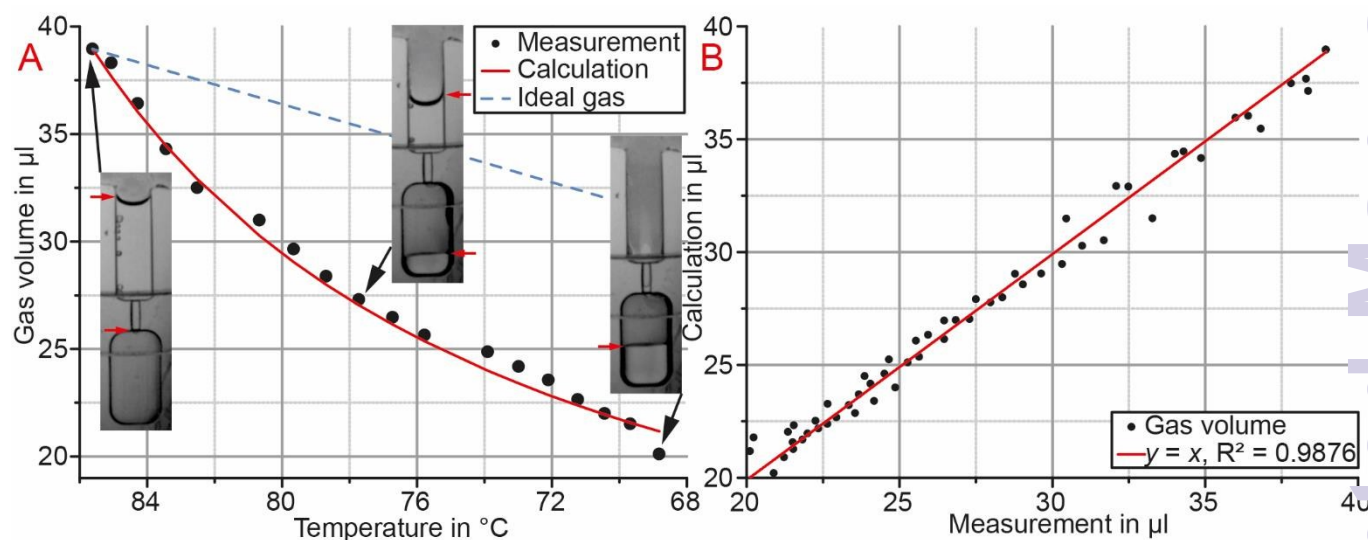
Fig. 6 Characterization of gas volume contraction in reaction cavities during cool down for centrifugo-thermopneumatic (CTP) two-stage aliquoting. A: Comparison of calculated and measured volume contraction inside a single reaction cavity over temperature decrease. Additional depiction of three corresponding stroboscopic images (red arrows illustrate liquid menisci). The dashed line (blue) compares CTP fluid control with ideal air volume contraction to illustrate the dominance of partial vapor pressure. B: Comparison of calculated and measured gas volume contraction for all measurements ( n = 3 ).
