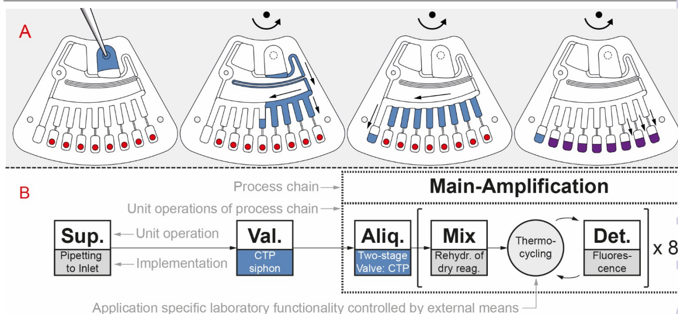
Fig. 1 Illustration of workflow for geometrically multiplexed real-time PCR. A: Sample liquid is supplied to the disk segment “GeneSlice” by pipetting to the sample inlet, which is then sealed. The GeneSlice aliquots the sample liquid into eight reaction cavities with pre-stored primers and probes (red). B: Schematic representation of microfluidic process chain (Sup.: sample or reagent supply; Val.: valving; Aliq.: aliquoting; Mix: mixing; Det.: detection) 4 . The process is driven by novel centrifugo-thermopneumatic (CTP) siphon valving and CTP two-stage aliquoting (blue) to be compatible with the off-the-shelf thermocycler Rotor-Gene Q (QIAGEN, Hilden, Germany).
