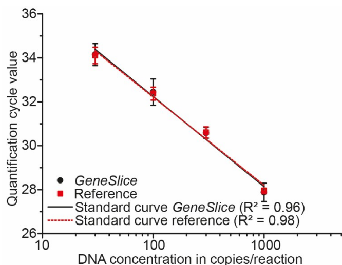
Fig. 7 Mean quantification cycle ( C_q ) values obtained from real-time PCR with 30, 100, 300, and 1000 copies/reaction in GeneSlices and reference reactions in conventional PCR tubes with corresponding standard deviations.
