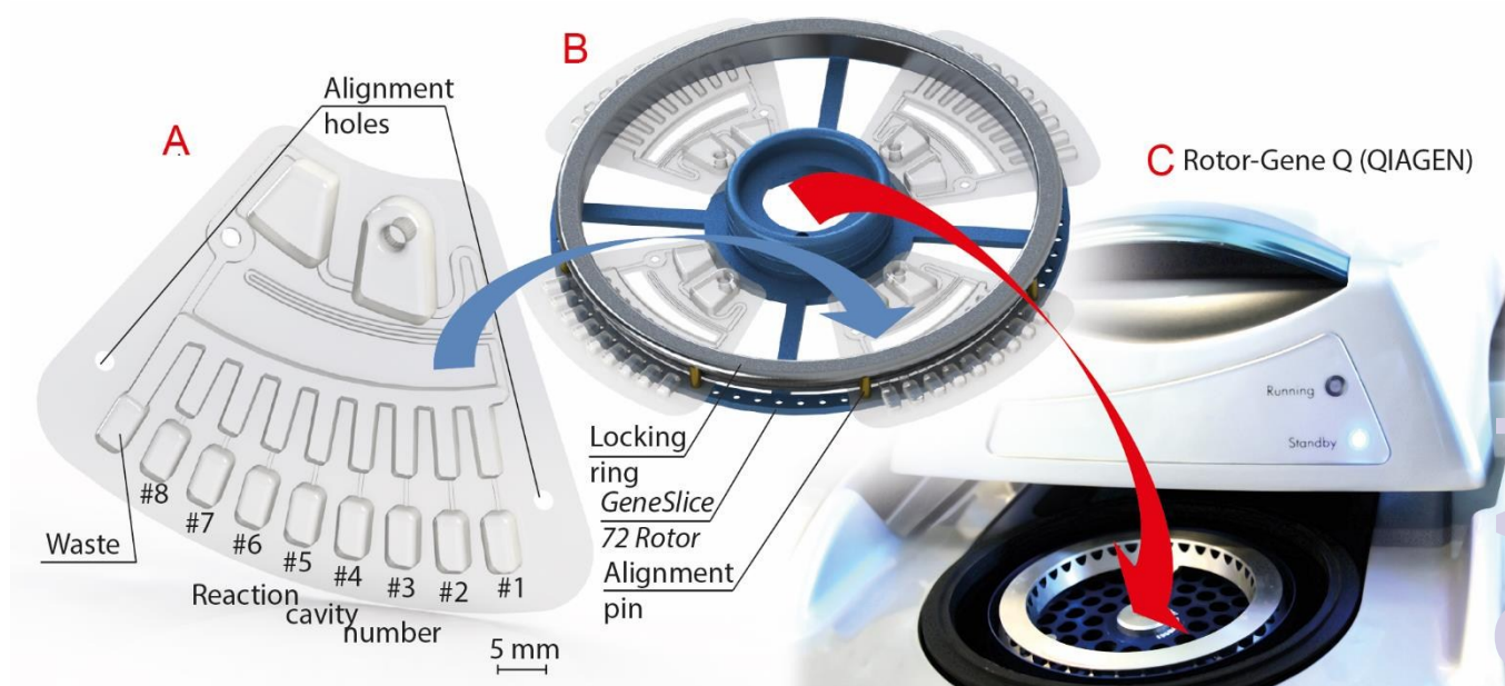
Fig. 5 Workflow of insertion of microfluidic disk segment “GeneSlice” into an off-the-shelf Rotor-Gene Q (RGQ, QIAGEN, Hilden, Germany). A: Overview of GeneSlice . B: Custom GeneSlice 72 Rotor , which holds up to four GeneSlices . Alignment pins are provided by the GeneSlice 72 Rotor for precise alignment of the GeneSlice reaction cavities to the fluorescence detector inside the RGQ. GeneSlices are held into place during processing by a locking ring. C: Depiction of its insertion into an RGQ instead of the depicted standard tube rotor.
