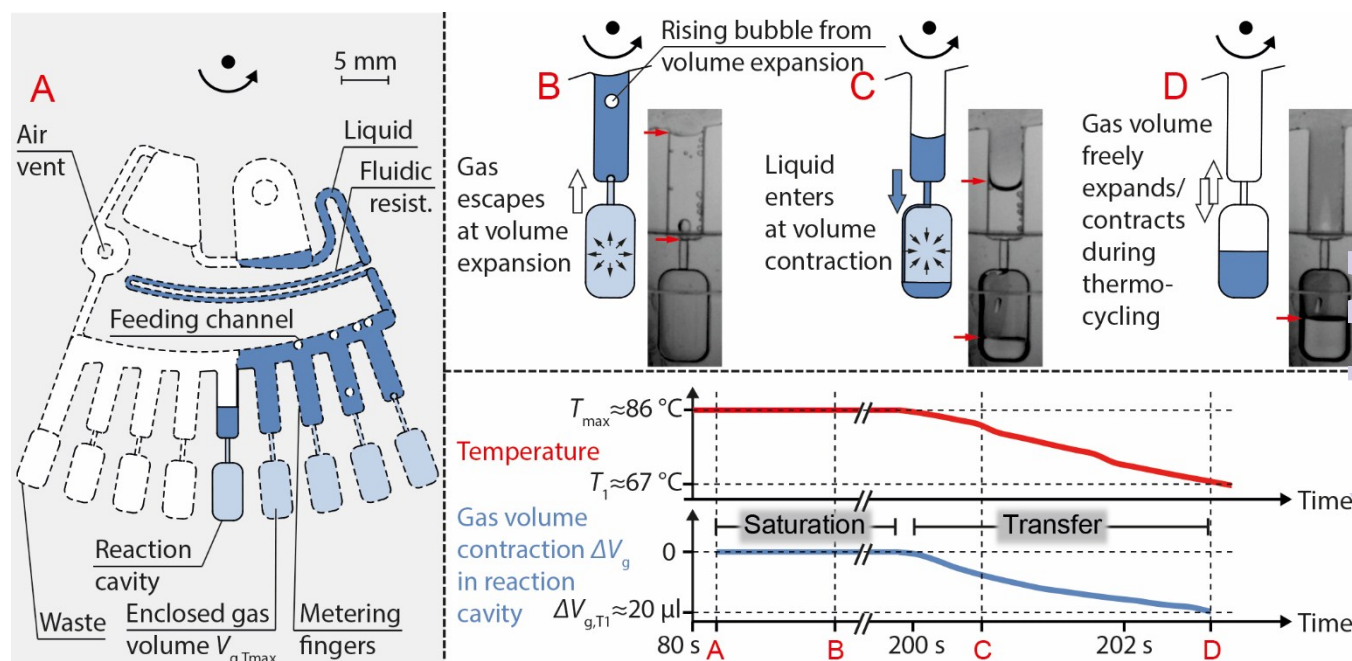
Fig. 4 Functional principle of centrifugo-thermopneumatic (CTP) two-stage aliquoting. A: CTP two-stage aliquoting comprises a feeding channel with metering fingers, which are connected to dead-end reaction cavities via narrow channels. During metering gas volumes V_{g,T_{\max}} inside each reaction cavity are enclosed. B: Due to saturation of the gas volumes inside the reaction cavities with partial vapor pressure, bubbles are formed and escape through the metering fingers. C: Temperature decrease from T_{\max} to T_1 contracts the gas volume according to eqn (6), which aspirates liquid from the metering fingers into the reaction cavities. D: Once the entire aliquot is transferred, the gas volume is vented again and is free to expand and contract during subsequent thermocycling for PCR. Liquid menisci are marked with red arrows. Temperature and gas volume contraction at each depicted stage (A-D) are plotted over time. The entire operation takes place at constant rotational speed of 400 RPM. Quantitative values in the plots are given for the microfluidic cartridge detailed in the “design and fabrication” section.
