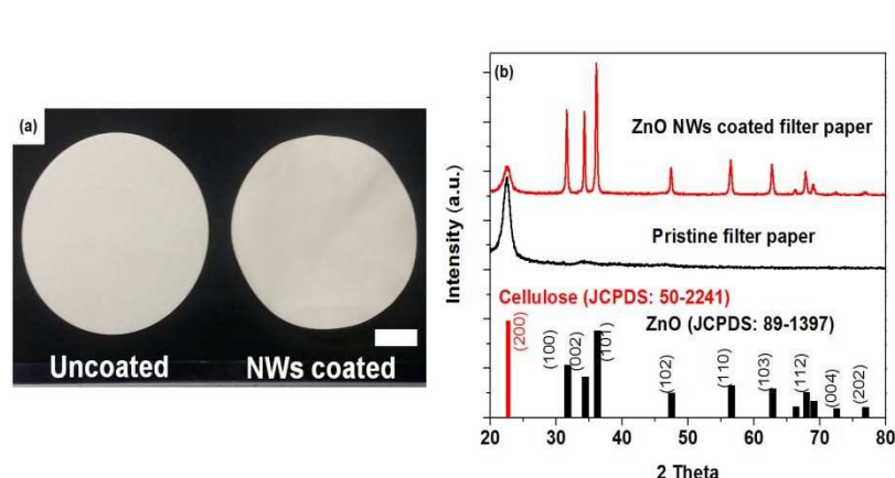
Fig. 2 (a) Optical images of filter paper before (left) and after (right) ZnO NWs coating (scale bar is 2 cm). (b) XRD pattern of uncoated (pristine) and ZnO NWs coated filter paper. (c), (d) secondary electron SEM images of uncoated (pristine) cellulose filter paper with fiber network. (e), (f) secondary electron SEM images of ZnO NWs coated cellulose fibers.
