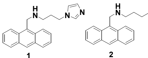
Fig. 1. Structures of 9- N -alkylaminomethylantracene probes 1 and 2 .
