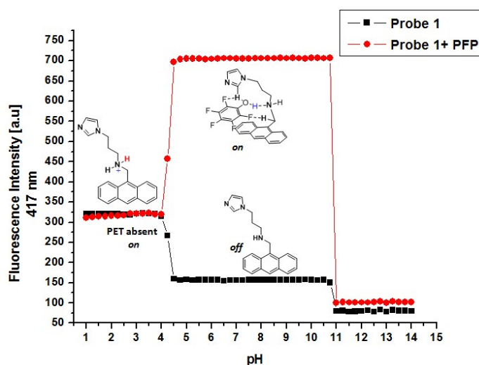
Fig. 6. The pH-dependent fluorescence studies of probe 1 (20 \mu M) alone and in the presence of 1.0 eq. of PFP (20 \mu M) from pH 1 to 14, \lambda_{ex} = 365 nm and \lambda_{em} = 417 nm in EtOH.
