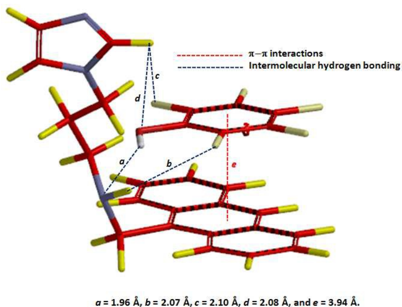
Fig. 7. Energy-minimised structure of 1 •PFP using B3LYP/6-31G* method in EtOH (implicit) medium.
