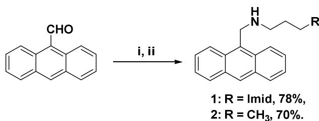
Scheme 1. Synthesis of 9- N -alkylaminomethylanthracene probes 1 and 2 .
