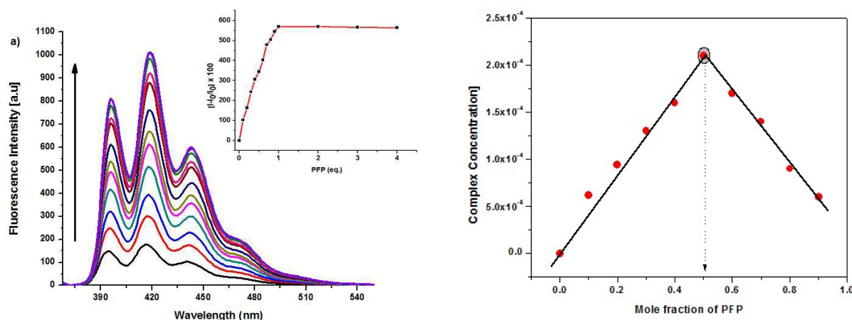
Fig. 4. (a) Fluorescence titration spectra of probe 1 (20 \mu\text{M} ) with PFP in EtOH. The inset shows the molar ratio plots of the fluorescence enhancement: \lambda_{ex} = 365 \text{ nm} and \lambda_{em} = 417 \text{ nm} . (b) Job's plot of probe 1 (20 \mu\text{M} ) with PFP (20 \mu\text{M} ) in EtOH: \lambda_{ex} = 365 \text{ nm} and \lambda_{em} = 417 \text{ nm} .
