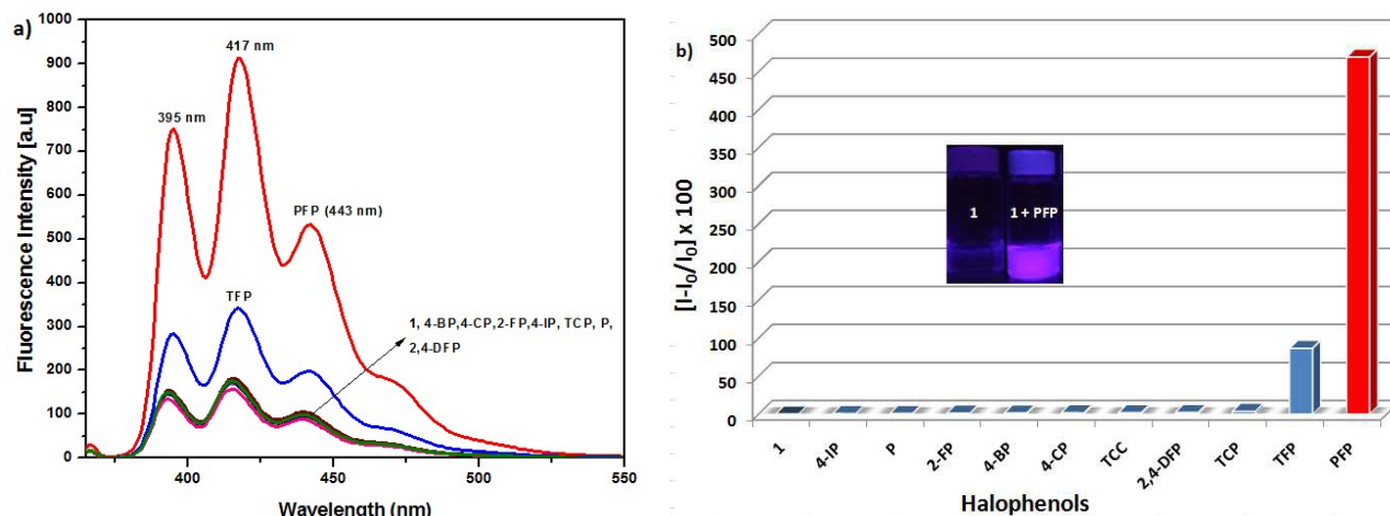
Fig. 3. (a) Fluorescence spectra of probe 1 (20 μM) in the presence of various halophenols (200 μM, each): \lambda_{ex} = 365 nm; (b) Relative fluorescence enhancement ratio [(I-I_0/I_0) \times 100] intensity bar graph of probe 1 (20 μM) with various halophenols (200 μM) in EtOH: \lambda_{ex} = 365 nm and \lambda_{em} = 417 nm. The inset figure shows the fluorogenic responses of probe 1 and 1 •PFP complex.
