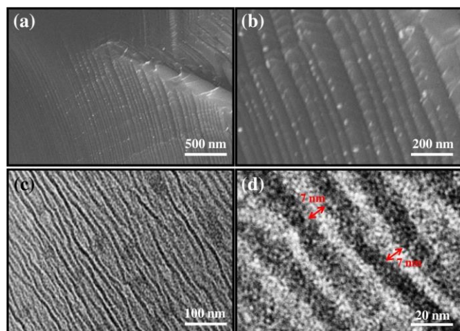
Fig. 4: Controlling the crystalline structure and morphology of UrCy-PPG. SEM (a, b) and TEM (c, d) images showing the lamellar structures of annealed UrCy-PPG; the width of the lamellar structures is indicated by arrows in (d).
