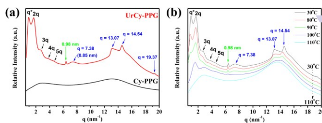
Fig. 3: Long-range ordering of supramolecular polymers induced by complementary interactions. (a) One-dimensional XRD data for Cy-PPG and UrCy-PPG recorded at 30 °C. (b) Variable-temperature XRD data for UrCy-PPG recorded at a range of temperatures from 30 °C to 110 °C at 3 °C/min.
