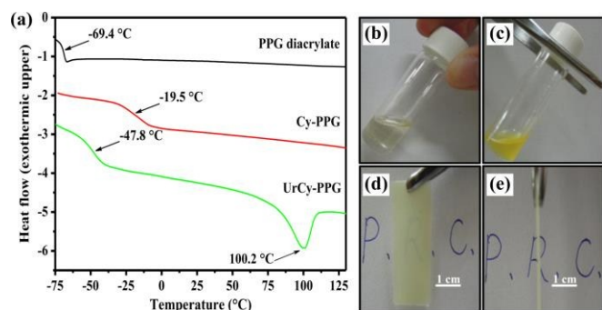
Fig. 2: Characterization of self-assembly behavior in the bulk state. (a) DSC curves for cytosine-functionalized PPGs and the controlled PPG diacrylate. Appearance of (b) PPG diacrylate, (c) Cy-PPG and (d, e) UrCy-PPG.
