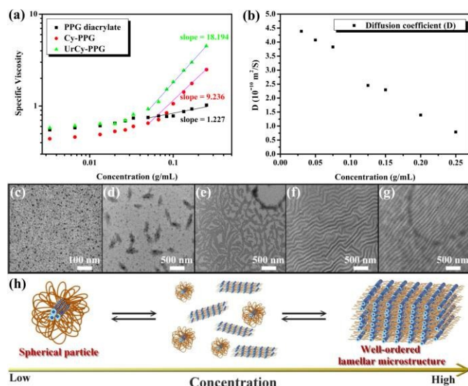
Fig. 1: Spontaneous formation of polymer-like features in toluene solution. (a) Plot of specific viscosity versus concentration in toluene at 25 °C for various polymers. (b) Plot of diffusion coefficient as a function of concentration for supramolecular polymerization of UrCy-PPG. TEM images of UrCy-PPG on carbon-coated copper grids at different concentrations: (c) 0.03, (d) 0.05, (e) 0.075, (f) 0.2 and (g) 0.35 g/mL. (h) Graphical representation of the hierarchical self-assembly of UrCy-PPG in solution.
