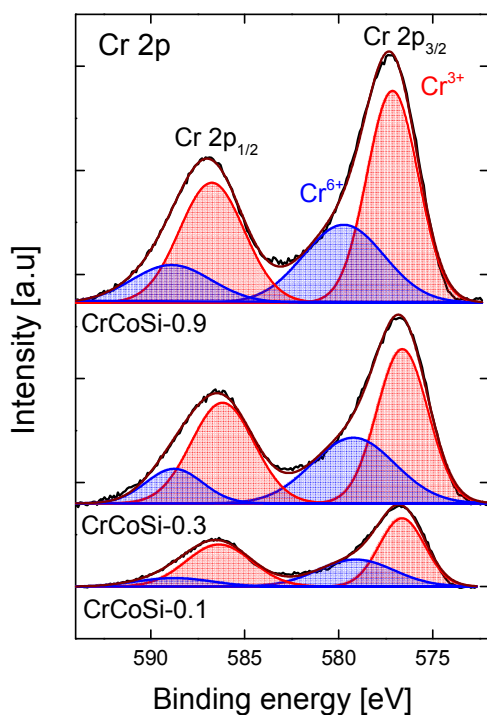
Fig. 7 Cr2p spectra recorded from CrCoSi samples with different Cr/Co (Cr/Co = 0.1, 0.3, 0.9) molar ratios.
