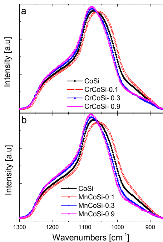
Fig. 8 FTIR spectra of all samples in the region 850-1300 \text{cm}^{-1}
