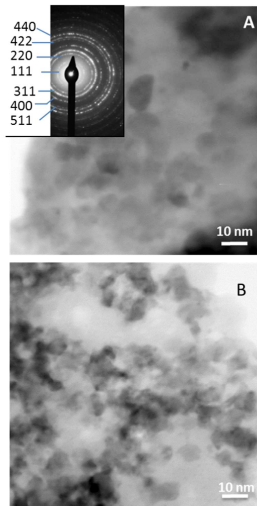
Fig. 4 XRD representative bright-field TEM images and electron diffraction pattern (insert) of the MnCoSi-0.1 sample of the sample (see Fig. S2).
