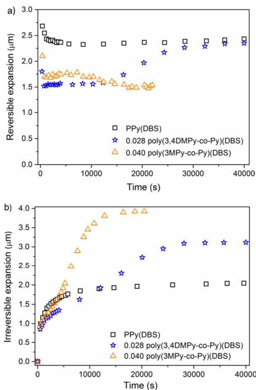
Fig. 7 a) The reversible expansion of PPy(DBS), 0.040 poly(3MPy-co-Py)(DBS) and 0.028 poly(3,4DMPy-co-Py)(DBS) with time. b) The irreversible expansion of PPy(DBS), 0.040 poly(3MPy-co-Py)(DBS) and 0.028 poly(3,4DMPy-co-Py)(DBS) with time.
