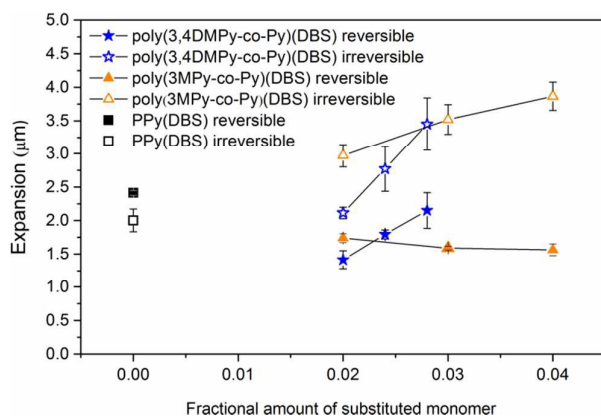
Fig. 8 The variation in maximum reversible and irreversible expansion in the stable state with increasing substituted monomer content ( n=3 ). Fraction 0.00 means PPy(DBS) homopolymer. Error bar = 1SD.
