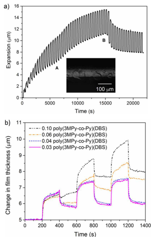
Fig. 5 a) A typical actuation profile for a 0.06 poly(3MPy-co-Py)(DBS) copolymer film. The profile displays very large increases in reversible and irreversible expansions. In region A deformation, like that shown in the inset, occurs. At point B delamination occurs. b) An overlay of the first three cycles of 0.03 to 0.10 poly(3MPy-co-Py)(DBS) copolymer films showing the existence of a 'threshold' fraction above which plastic deformation occurs.
