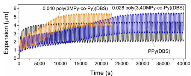
Fig. 6 Overlays showing a typical actuation sequences for 5 \mu\text{m} films of PPy(DBS), 0.040 poly(3MPy-co-Py)(DBS) and 0.028 poly(3,4DMPy-co-Py)(DBS).
