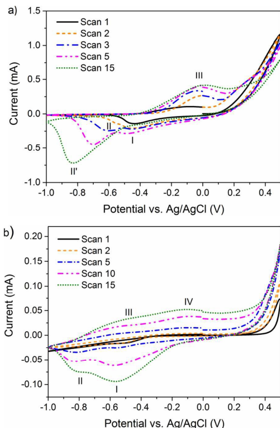
Fig. 3 Voltammograms for a) 3,4DMPPy(DBS) and b) 3MPPy(DBS) potentiodynamically synthesised at a gold working electrode employing 0.1M solutions of aqueous monomer and NaDBS electrolyte at a scan rate of 0.05 V/s.
