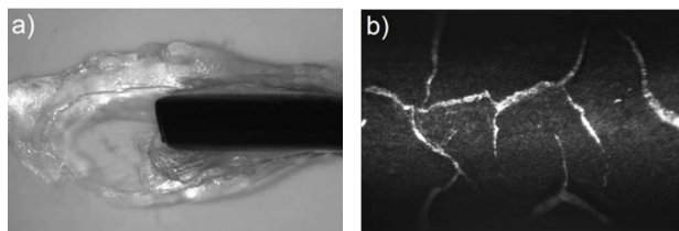
Fig. 4 a) The two phases formed during (black solid phase) and after (transparent phase) CV of 0.01 M 3,4DMPPy and 0.1 M NaDBS (aq) at a scan rate of 0.05 V/s. b) A highly fractured homopolymer film of 3MPPy(DBS) formed during actuation revealing the gold substrate.
