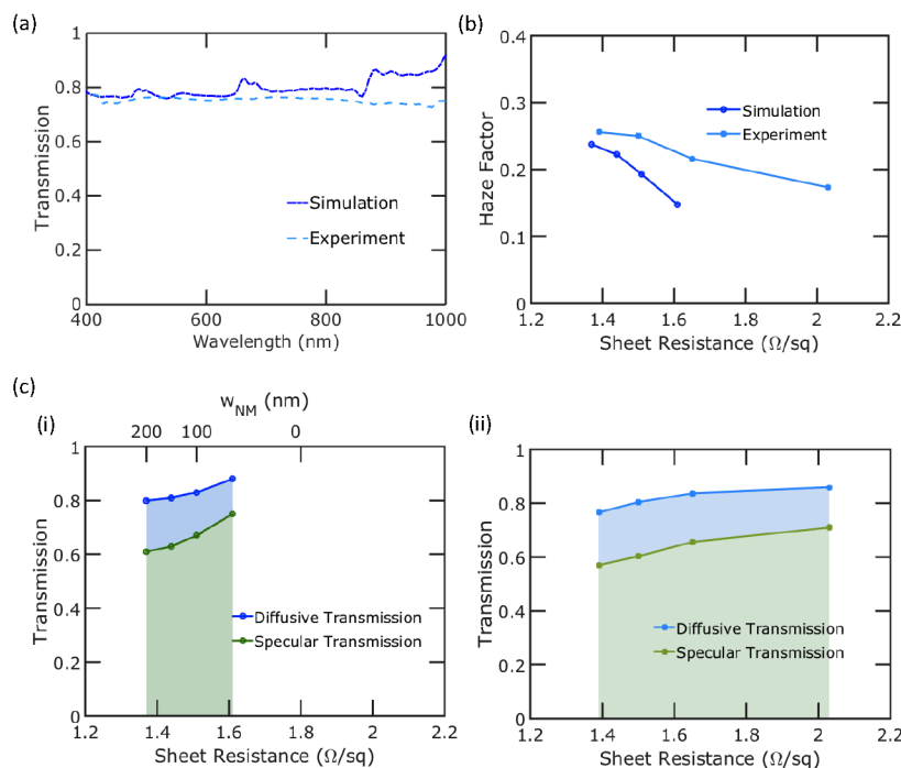
Fig. 3 (a) Diffusive transmission spectrum for Ag NM/MG with a_{NM} = 2000 nm, w_{NM} = 100 nm, t_{NM} = 30 nm, a_{MG} = 200 \mu\text{m} , w_{MG} = 5 \mu\text{m} , and t_{MG} = 1 \mu\text{m} obtained by simulation and experiment. (b) Haze factor as a function of sheet resistance for experimental and simulated samples with a_{MG} = 500 \mu\text{m} , w_{MG} = 5 \mu\text{m} , t_{MG} = 1 \mu\text{m} , a_{NM} = 2000 nm, t_{NM} = 20 nm, and various w_{NM} . (c) Diffusive transmission and specular transmission as a function of sheet resistance at \lambda = 550 nm for Ag NM/MG with different extends of haziness using (i) simulation and (ii) experiment. w_{NM} is varied from 200 to 50 nm in simulation to match the experimental geometry and is labelled accordingly. w_{NM} = 0 corresponds to that the sheet resistance is only contributed by Ag MG.
