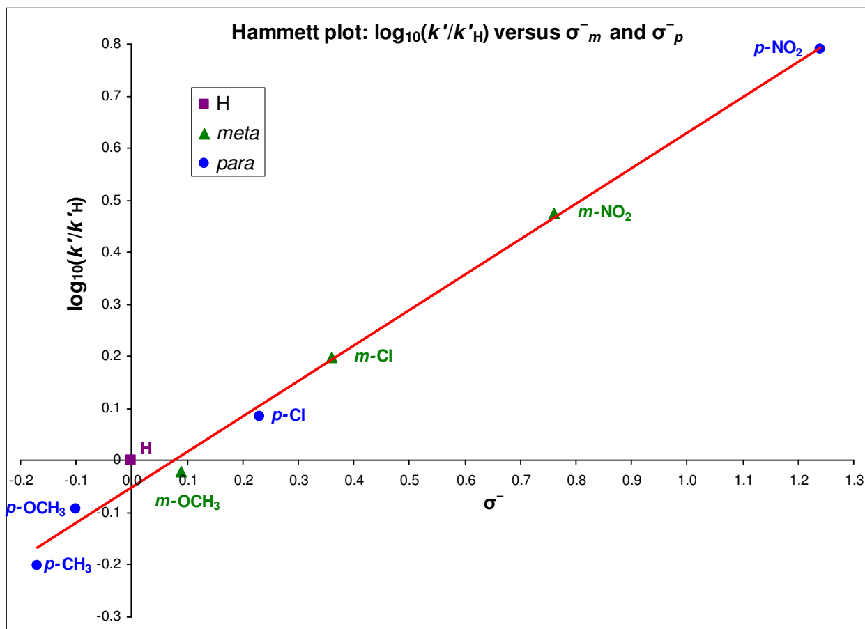
Figure 11. Hammett plot
