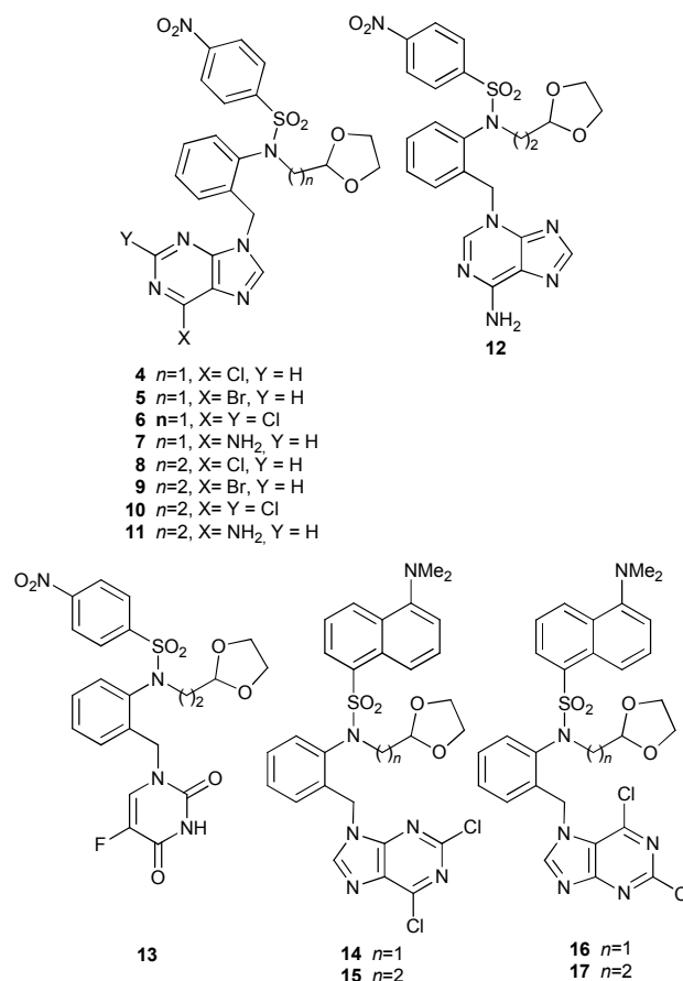
Figure 2. The fourteen molecules studied in this communication.
