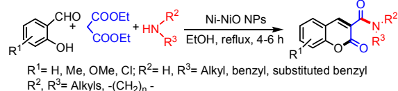
Scheme 1 Multi-component reaction of 2-hydroxybenzaldehyde, amine and diethyl malonate.
