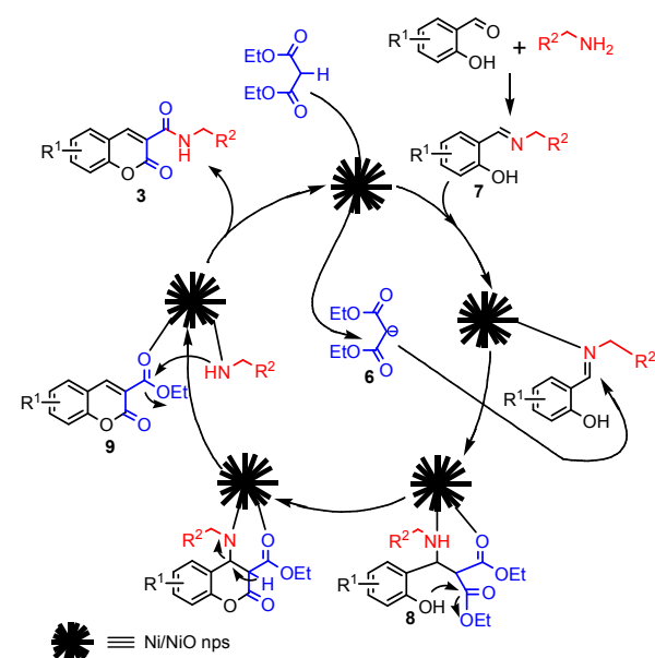
Scheme 2 Probable mechanistic pathway for multicomponent reaction of aldehyde, amine and DEM.
