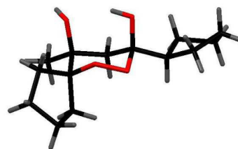
Figure 1: X-ray diffraction analysis of compound 2 .
