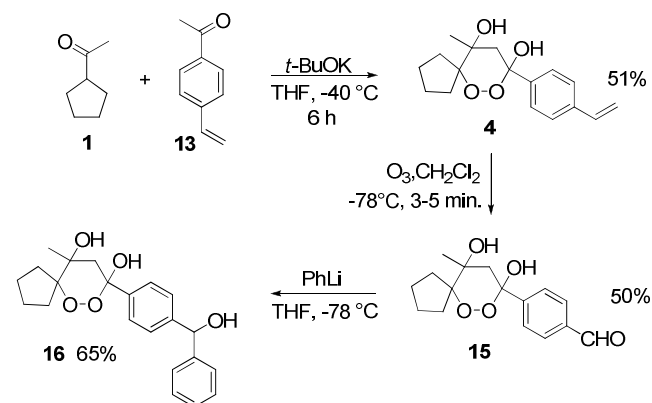
Scheme 4: Linking the endoperoxide structural unit to other structures via organometallic addition.
