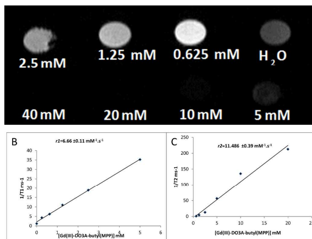
Fig. 1A) T_1 weighted image of Gd-DO3A-butyl-MPP at different concentrations varying from 0.625 mM–40 mM. Concentration range of 0.625–40mM of Gd-DO3A-butyl-MPP exhibited in MR studies, the effect being more marked at lower concentrations. At concentration as low as 0.625mM, enhanced contrast was obtained whereas darker image intensity was observed at higher concentration of the complex. 1B & C). In vitro MR measurement of the longitudinal and transverse relaxivity, r_1 and r_2 of Gd-DO3A-butyl-MPP with varying concentrations.
