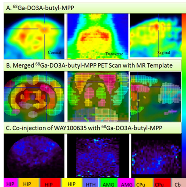
Fig 3. MicroPET images of Rat brain showing Coronal, transverse and sagittal sections respectively after the intravenous injection of 37 MBq of ^{68}\text{Ga} -DO3A-butyl-MPP. A. SD Rat depicting high accumulation of radioactivity in hippocampus, amygdala and Caudate Putamen. B. Coregistration of rat MRI atlas on the microPET scan for anatomical confirmation of the brain regions was done using PMOD and C. Blocking studies with WAY-100635.
