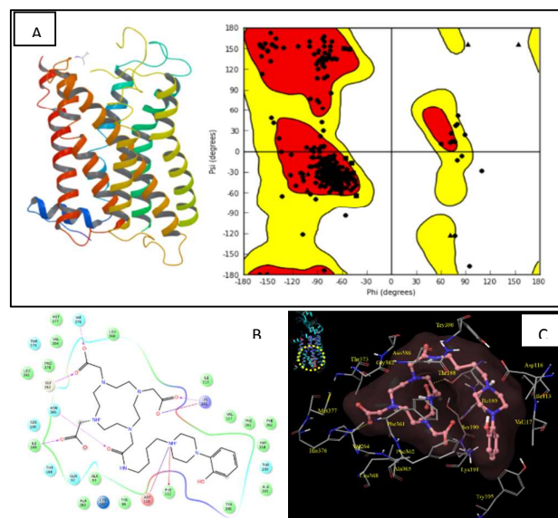
Fig. 8 (A) Model of the human 5-HT 1A receptor and Ramachandran Plot showing the transmembrane helices in different colours. (B) Two dimensional view of DO3A-butyl-MPP with 5-HT 1A receptor where green colored are hydrophobic, light blue are polar, red are negative and purple are positive charged residues. Pink lines are hydrogen bonds, red lines are \pi -cation interactions. (C) Three dimensional view of DO3A-butyl-MPP (pink carbon layout) at the binding pocket of 5-HT 1A homology modeled receptor. Yellow dashed lines are showing the hydrogen bonds.
