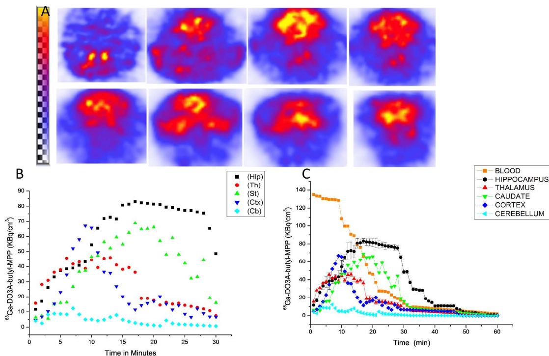
Fig. 2A. 0-30 minutes summation images of rat brain coronal microPET Scan depicting activity in different section (Slices) of the Brain. B. Time activity curve (TAC) of different regions for 30 minutes and C. TAC for 60 minutes post 68 Ga-DO3A-butyl-MPP injection in rat (n=5).
