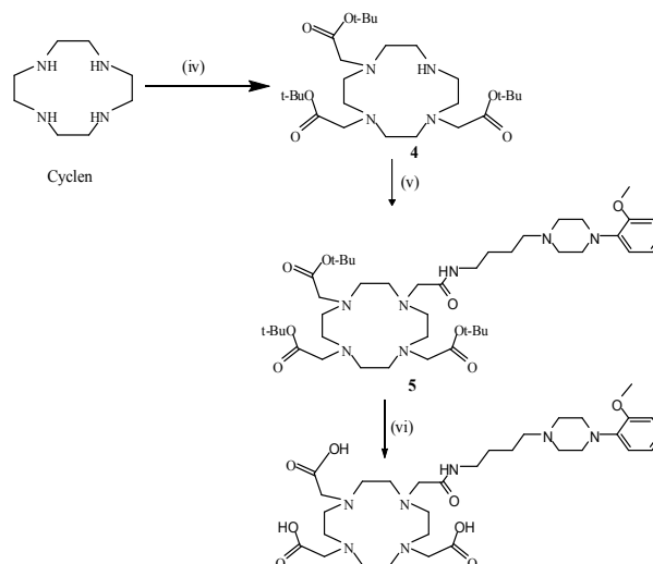
Scheme 1b Synthesis of 2,2',2''-(10-(2-(4-(4-(2-methoxyphenyl)piperazin-1-yl)butylamino)-2-oxoethyl)-1,4,7,10-tetraazacyclododecane-1,4,7-triyl)triacetic acid (6) Reagents and conditions: iv) ACN, NaHCO 3 , 0°C, tert-butylbromoacetate (v) ACN, 3, 70°C (vi) 20% TFA in DCM, 0°C.
