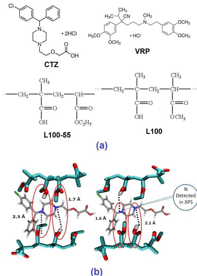
Fig. 1: (a) Chemical structures of the drugs and polymers, (b) Molecular modelling of CTZ with L100 (energy optimized to local minima at the B3LYP/6-31G* level and verified by frequency calculations using Gaussian09).
