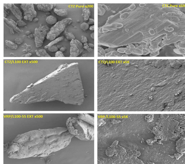
Fig. 2: SEM images of CTZ pure, CTZ/L100 and VRP/L100-55 extruded formulations.
