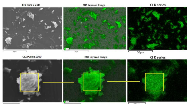
Fig. 3a: SEM-EDS mapping images of chlorine (Cl) atom detected on pure CTZ particles.
