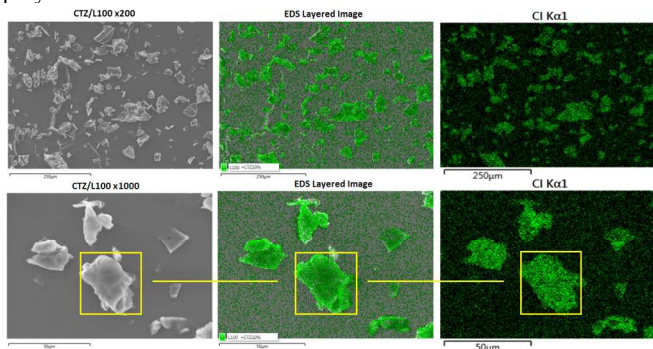
Fig. 3b: SEM-EDS mapping images of Cl atom detected on CTZ/L100 extruded formulations.
