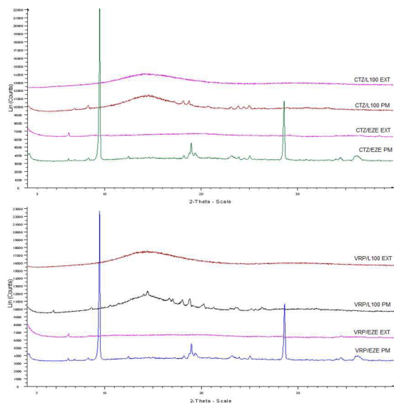
Fig. 5: XRD diffractograms of CTZ and VRP loaded physical mixtures (PM) and extruded formulations (EXT).
