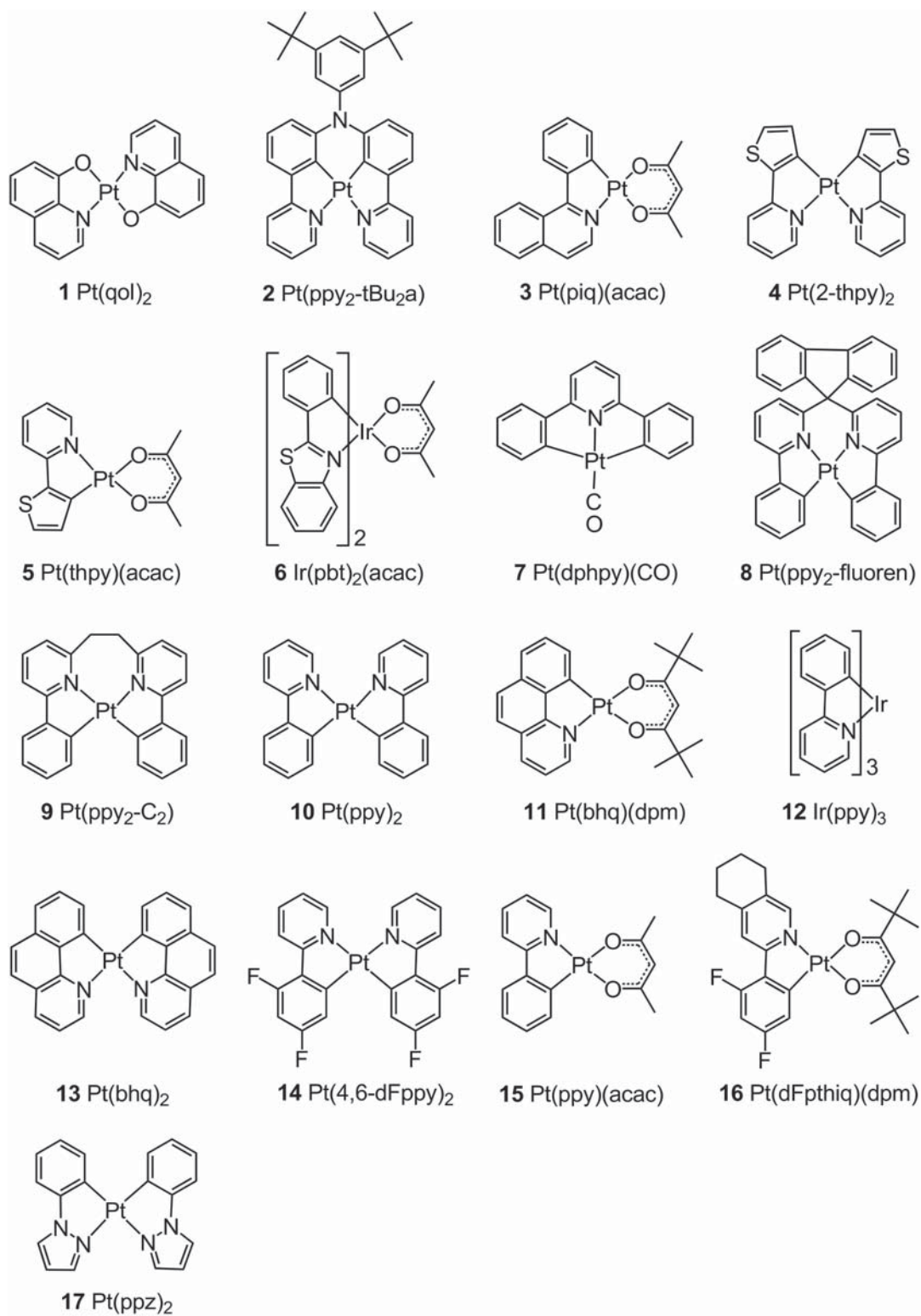
Figure 1: Chemical structures of compounds discussed. Complexes 11 and 13 are occasionally also abbreviated as Pt(bzq)(dpm) and Pt(bzq) 2 , respectively.
