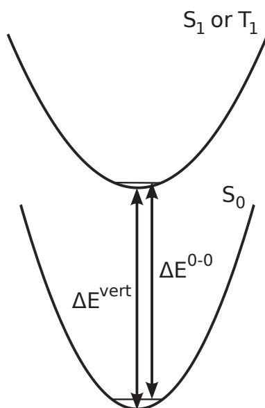
Figure 2: Potential energy surfaces for ground and excited states indicating the key quantities calculated. Depicted is a scenario with vanishing excited state relaxation.
