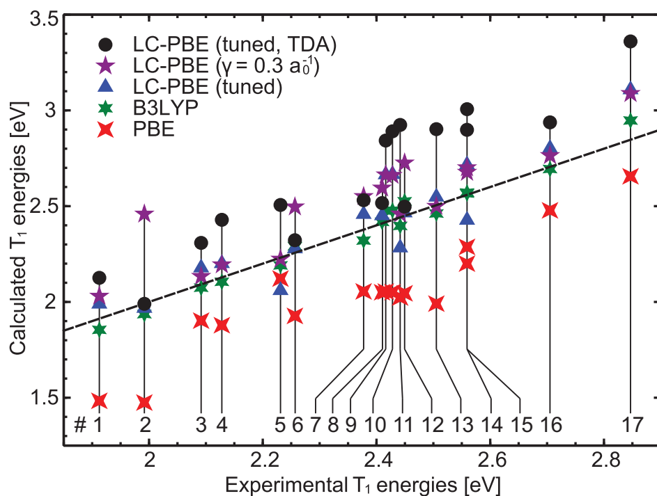
Figure 3: Calculated versus experimentally determined triplet emission energies ( \Delta E_{T_1}^{0-0} ) for various exchange-correlation functionals. The dashed line indicates perfect agreement. The stated numbers correspond to the complexes depicted in Figure 1.
