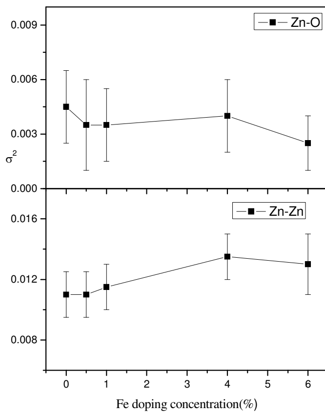
Fig. 11 Variation of Debye-Waller factor of Zn-O shells and Zn-Zn shells with change in doping concentration.
