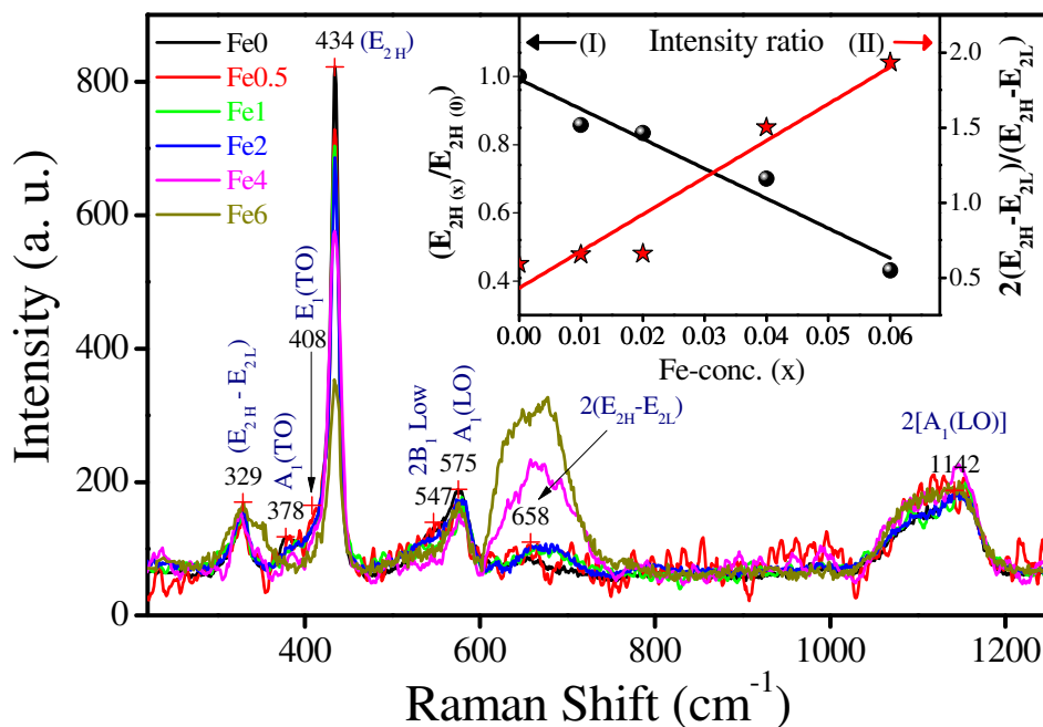
Fig. 13 Room-temperature Raman spectra of \text{Zn}_{1-x}\text{Fe}_x\text{O} ( 0 \leq x \leq 0.06 ) nanoparticles. Inset of figure shows the variation of the (E_{2H}) peak with Fe-concentration ( x ) with respect to its pure ZnO value. The inset shows the variation of the ratios E_{2H(x)}/E_{2H(0)} (curve I) and 2(E_{2H} - E_{2L})/(E_{2H} - E_{2L}) (curve-II) with x respectively .
