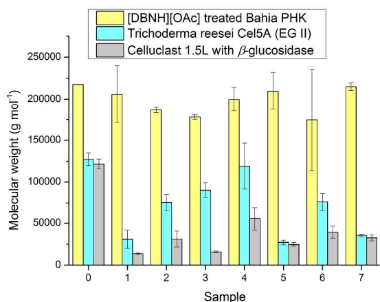
Figure 8. Weight averaged molecular masses ( M_w ) of enzymatically hydrolysed untreated and [DBNH][OAc]-treated samples. Reference sample M_w s are in yellow, total hydrolysis (Celluclast 1.5L supplemented with \beta -glucosidase) M_w s in grey and partial hydrolysis (Trichoderma reesei Cel5A) M_w s in cyan. The hydrolysis temperature was 45 °C, the time 24 h and the hydrolysis medium 50 mM citrate buffer at pH 5.0
